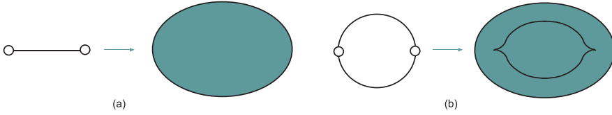
Figure 2: Associations of a network N to a planar portrait \mathcal{P}_f
