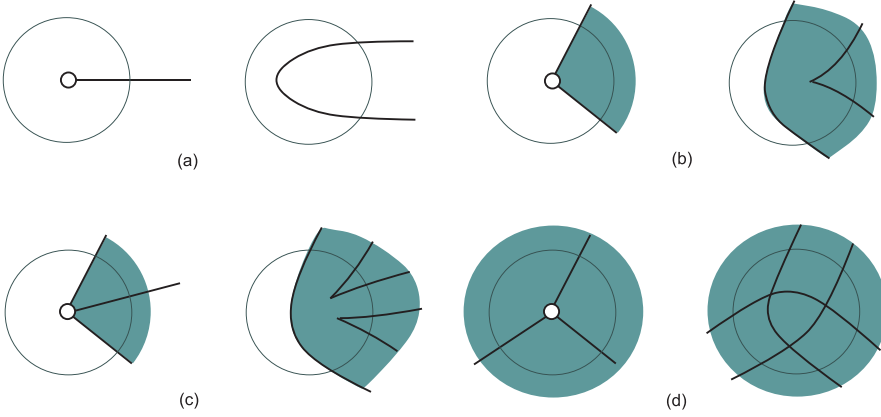
Figure 1: Association at a node: N (left) and D_f (right)
