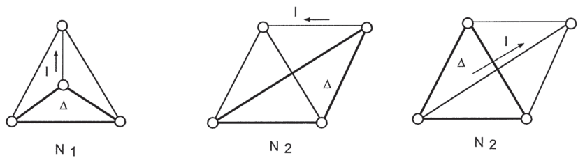
Figure 9: I -moves of \Delta
