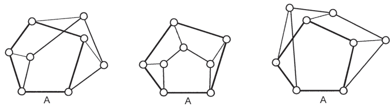
Figure 8: Various I -moves of a pentagon facet (bold)
