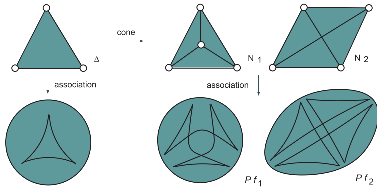
Figure 5: Cone over \Delta implies planar portraits of \mathbb{R}P^3 associated with the two representations N_1, N_2 of the network K_4 of blocks of \mathbb{R}P^3
