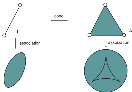
Figure 3: Cone over I implies a planar portrait of kP^2 associated with the network \Delta of blocks of kP^2
