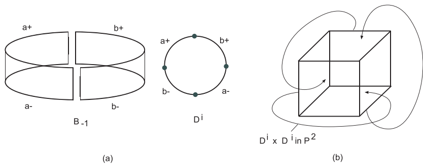
Figure 4: Block decomposition of kP^2 into three D^i \times D^i
