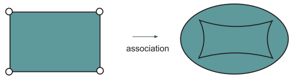
Figure 7: An I -product of I and its associated planar portrait \mathcal{P}_f of S^a -bundle over S^b .
