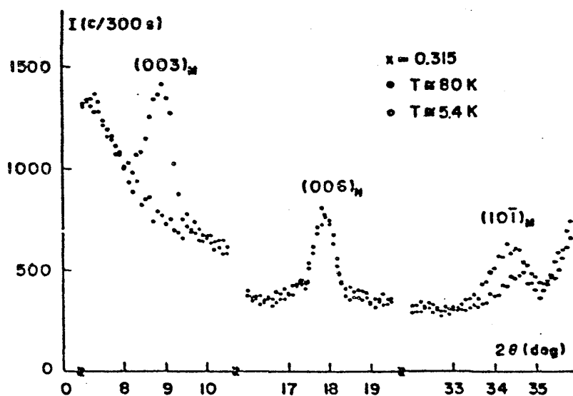
Fig. 6. Powder diffraction patterns for the x=0.315 sample obtained at T \approx 80 K and at T \approx 5.4 K.
