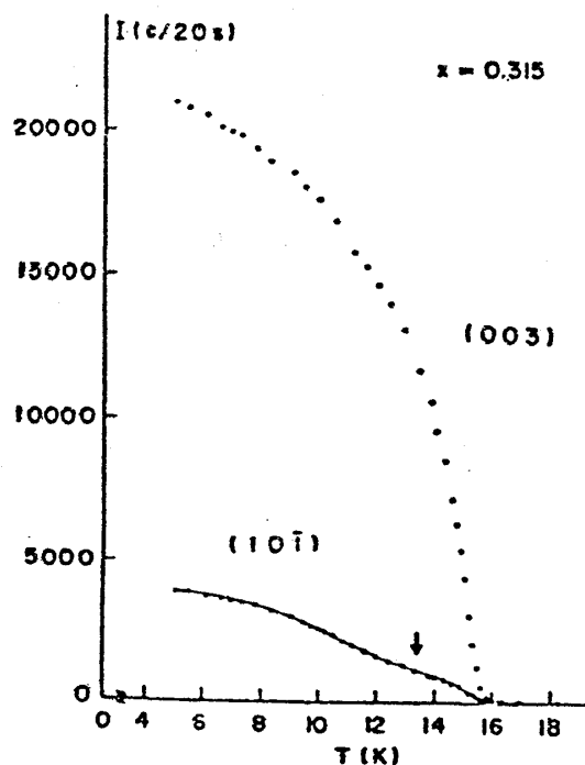
Fig. 5. Intensities of the (003) and (10\bar{1}) magnetic reflections observed near the tetracritical concentration ( x=0.315 ) are plotted as functions of temperature. The intensity of the (10\bar{1}) reflection decreases with increasing temperature in two steps, below and above about 13.3 K.
