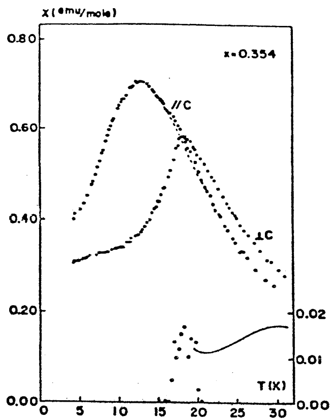
Fig. 1. Temperature dependence of the susceptibilities in an x=0.354 single crystal. The anomalous part of the susceptibility along the c -axis is shown at the lower part of this figure with the ordinate multiplied by ten.
