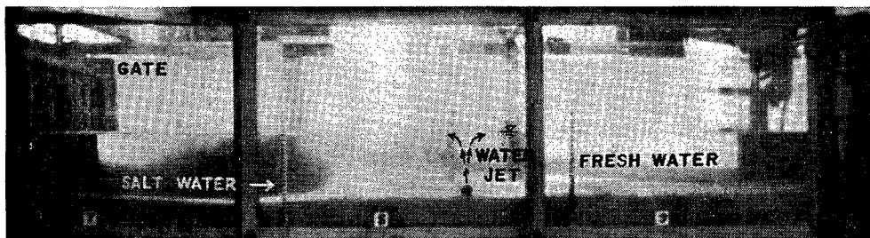
Photo. 1 Salt water wedge intruding through the gate.
