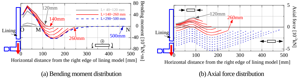
Figure 9. Mechanical behavior of the FRSP in the model experiment (Numerical result)
