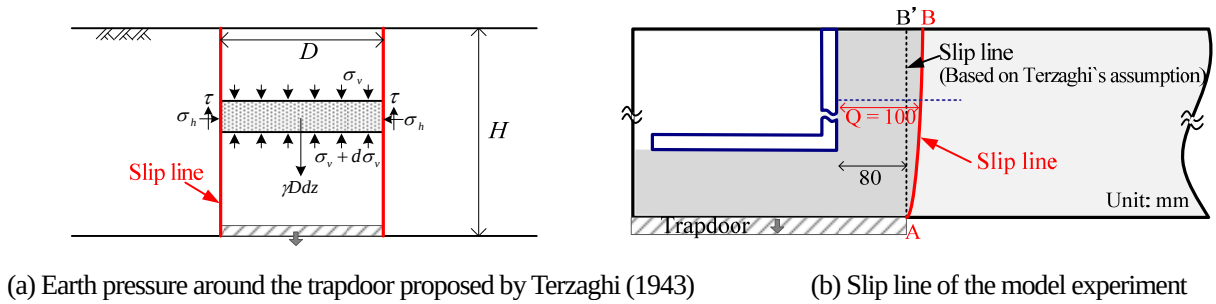
Figure 11. Slip line occurring due to lowering of the trapdoor
