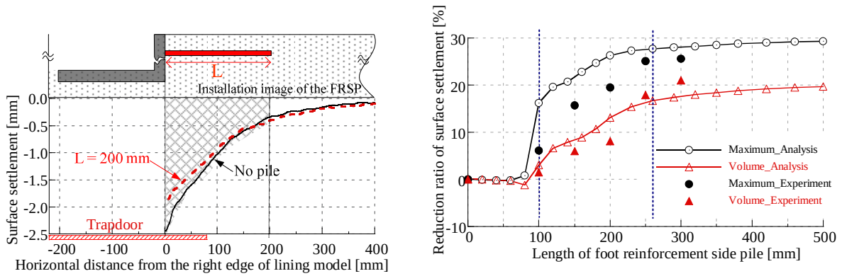
Figure 6. Influence of the length of the FRSP on surface settlement
