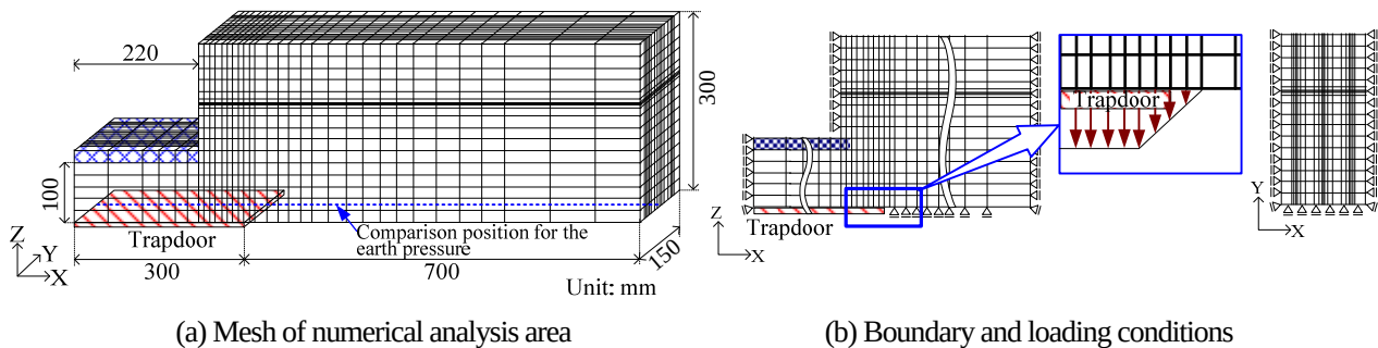
Figure 4. Mesh and the boundary conditions of the numerical analysis of model experiment
