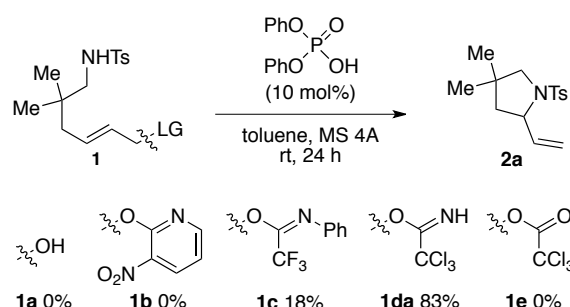
Scheme 1: Screening of leaving groups. The reactions were performed with 1 (0.1 mmol), (\text{PhO})_2\text{P}(\text{O})\text{H} (0.01 mmol), and MS 4A (50 mg) in toluene (0.4 mL). Isolated yields of 2a are shown.
