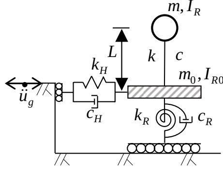
Fig.1 Swaying-rocking model subjected to free-field ground motion
