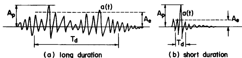
Fig. 1. Ground Motion Accelerograms and Illustration of EQA.
