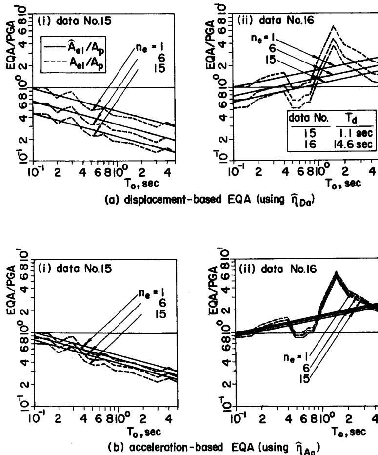
Fig. 18. Examples of Statistical Estimates for EQA, (soil condition 2; \mu=3 , q=1 ).
