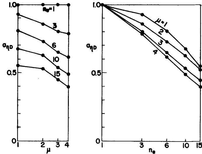
Fig. 13. Dependence of a_{\eta D} on \mu and n_e , ( q=1 ).
