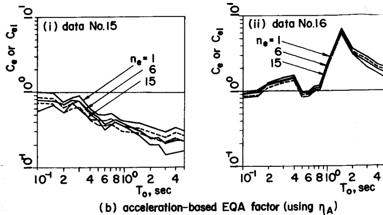
Fig. 7. Examples of EQA Factor (soil condition 2; \mu=3 , q=1 ).
