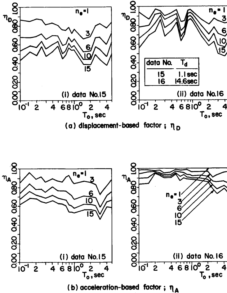
Fig. 6. Examples of Effective Response Factor \eta . ( \mu=3 , q=1 )
