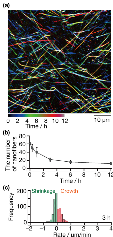
Figure 2. (a) Overlay of time-series CLSM images using a temporal color code. (b) Time course of the number of nanofibers. The data represent the mean \pm standard deviation ( n = 4 ). (c) Histogram analysis of the growth and shrinkage rate at 3 h. The shrinkage rate was shown as a negative value.
