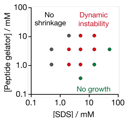
Figure 4. Phase diagram as a function of concentrations of the peptide hydrogelator and SDS.
