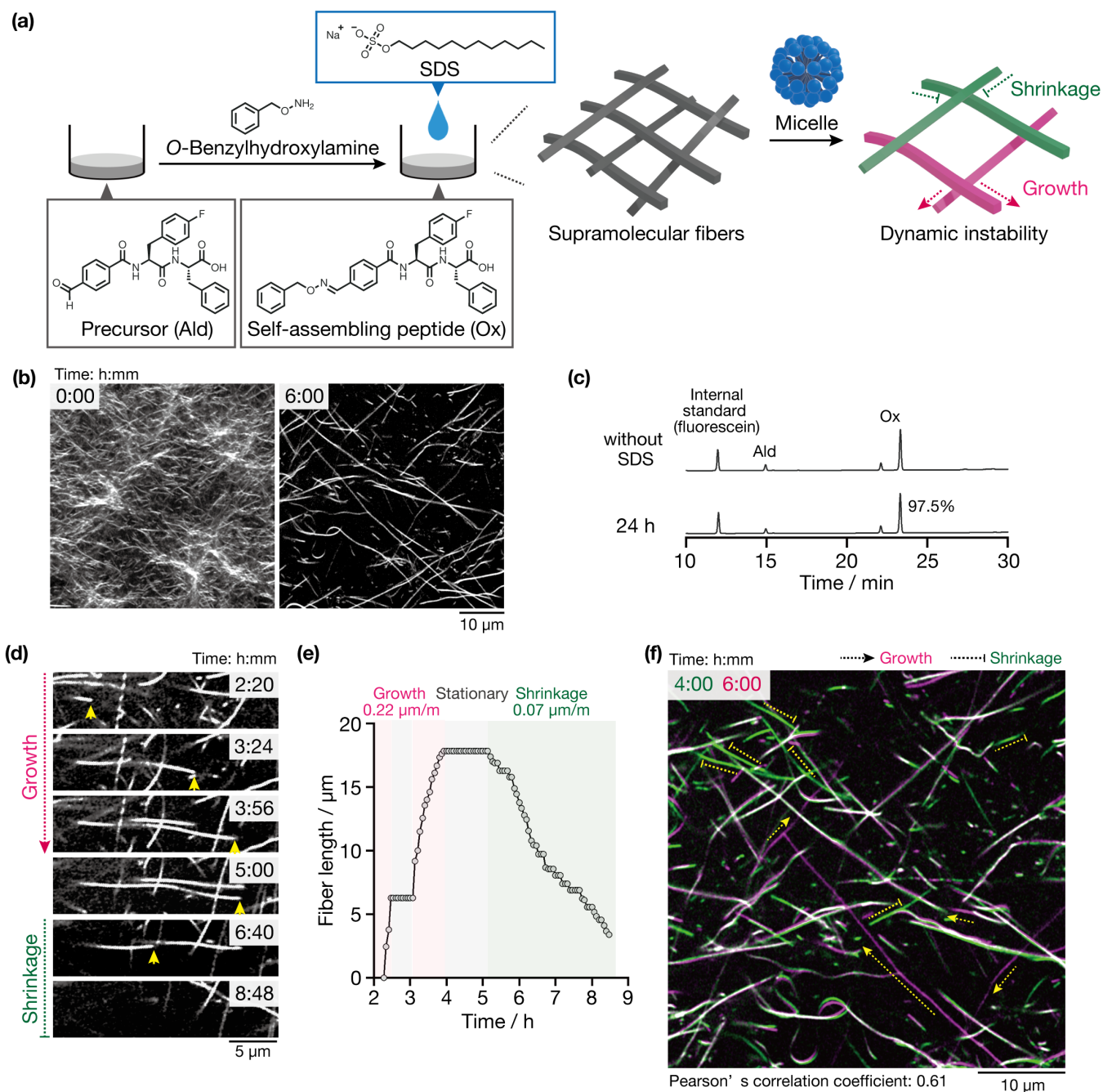
Figure 1. (a) Emergence of dynamic instability by hybridizing synthetic supramolecular fibers with surfactant micelles. (b) CLSM images and (c) HPLC charts before and after addition of SDS micelles. (d) CLSM images and (e) time course of single fiber dynamics. (f) Overlay of CLSM images at different time points (green: 4 h, magenta: 6 h). Condition: [Ald] = 3.6 mM, [O-benzylhydroxylamine] = 3.6 mM, [SDS] = 5.0 mM, [fluorescent probe] = 4.0 \mu\text{M} in 100 mM MES, pH 7.0, 30 ^{\circ}\text{C} .
