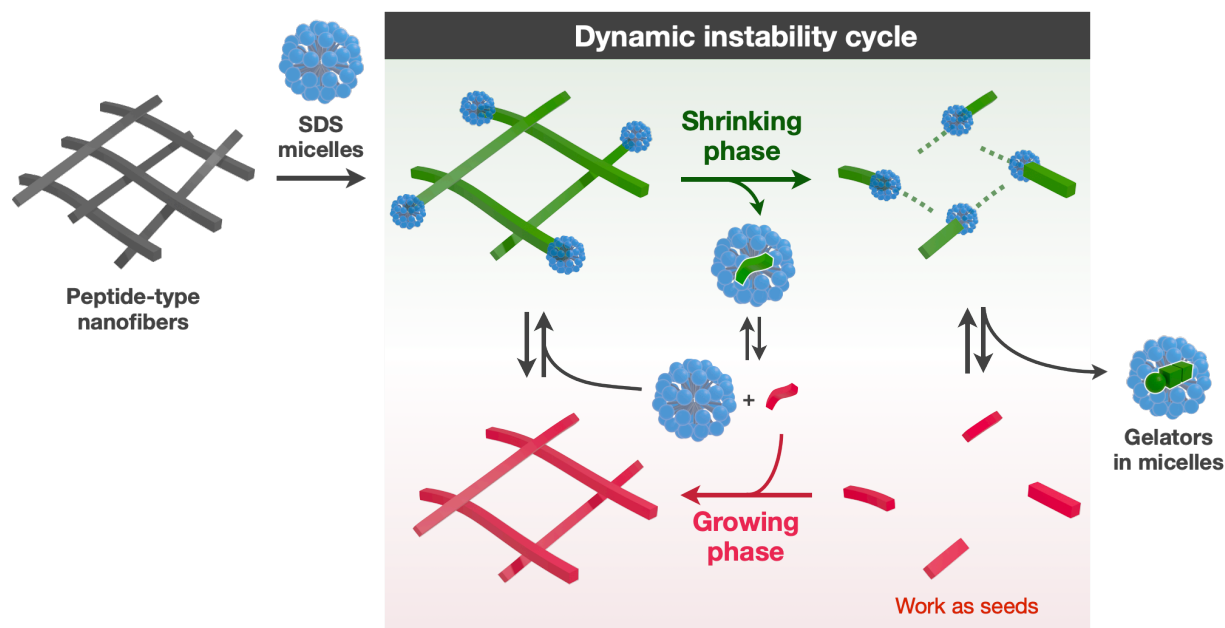
Figure 5. Plausible mechanism of synthetic dynamic instability of supramolecular nanofibers and surfactant micelles. Interaction strength between peptide fibers/aggregates and SDS micelles may be dependent on the fiber length, so that some of peptide aggregates are released from micelles followed by the fiber regrowth.
