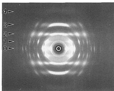
Figure 2. X-ray fiber pattern of the stereocomplex of PLLA and PDLA. The fiber axis is vertical. Figures on the left side show the order of layer line.
