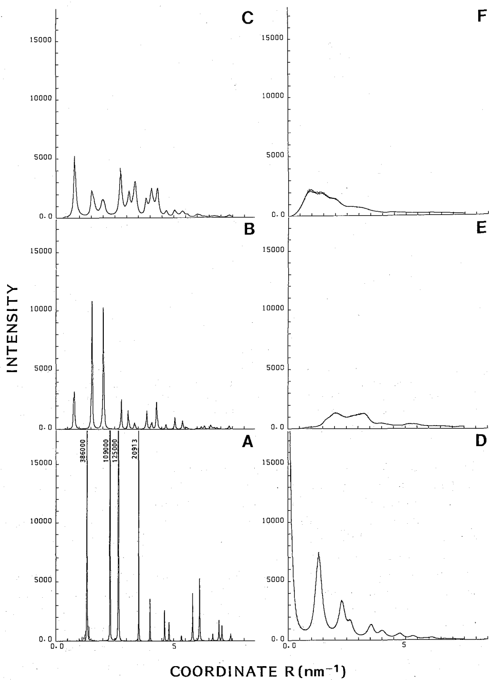
Figure 7. Patterns of A to F shows the calculated X-ray diffraction profiles on the zeroth to fifth layer line, respectively.
