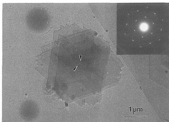
Figure 9. Electronmicrograph of the solution-grown lamella of the complex of PLLA and PDLA and the corresponding electron diffraction pattern. Arrows indicate the positions of the axes of the screw dislocations.
