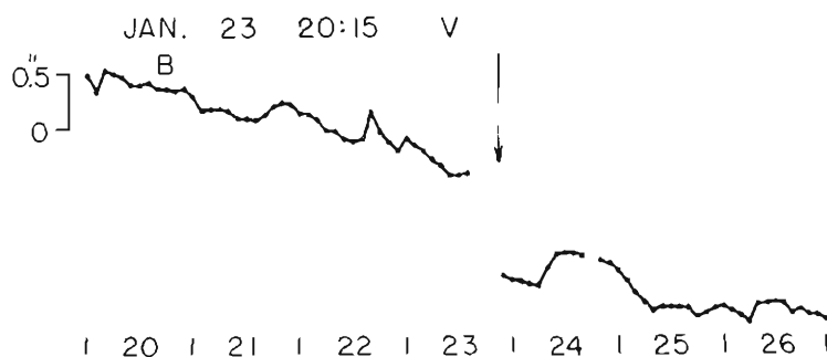
Fig. 7. Ground tilt observed before and after the earthquake on Jan. 23, 20h15m, 1966 ( M=4.6^{21} ).
