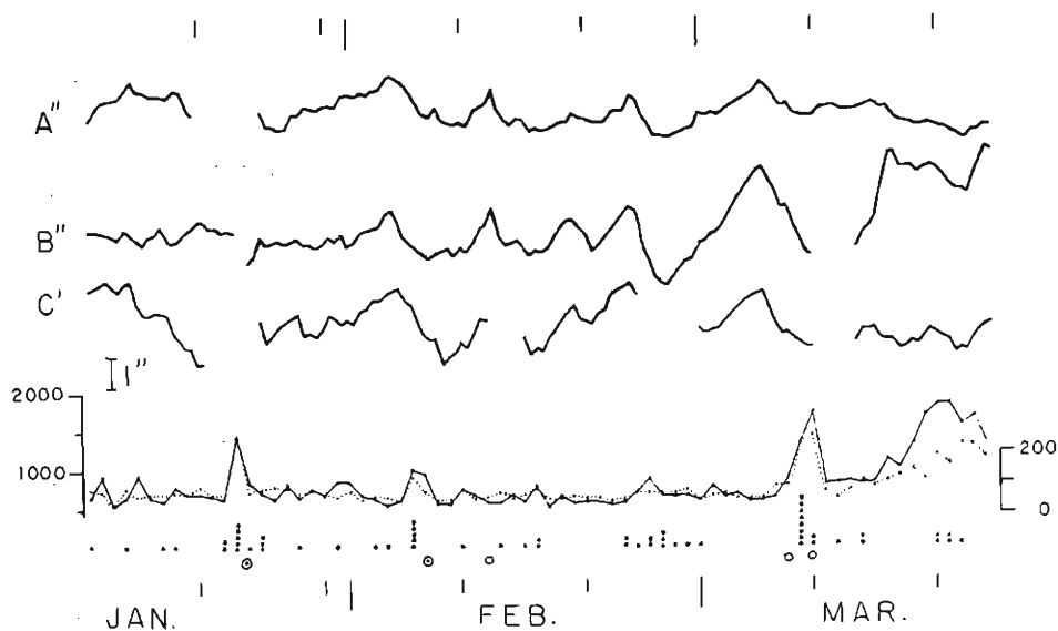
Fig. 5. Secular changes of the ground tilt corrected in regard to temperature influence and monotonous drift, and daily numbers of earthquakes (Reproduced from the Zishin Kazan Gaikyō 1) ).
