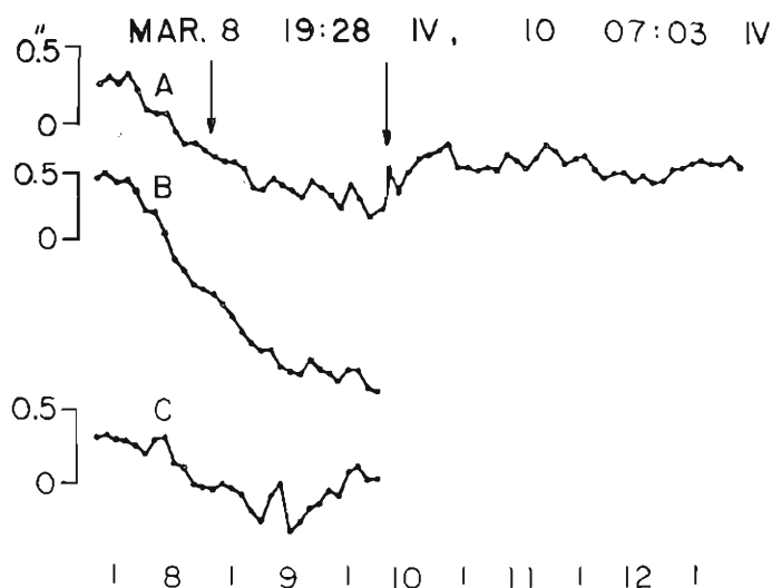
Fig. 10. Ground tilt observed before and after the earthquake on Mar. 8, 19h28m, 1966 ( M=4.5^{23} ).
