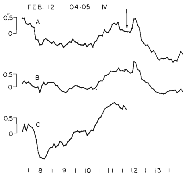
Fig. 9. Ground tilt observed before and after the earthquake on Feb. 12, 04h05m, 1966 ( M=4.6^{23} ).
