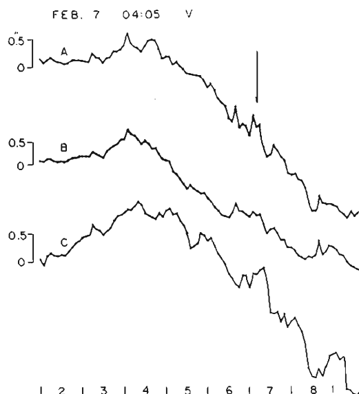
Fig. 8. Ground tilt observed before and after the earthquake on Feb. 7, 04h05m, 1966 ( M=4.4^{21} ).
