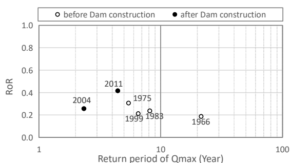
Fig. 6 Historical changes in riverbed environment at the downstream of Ootaki Dam.
