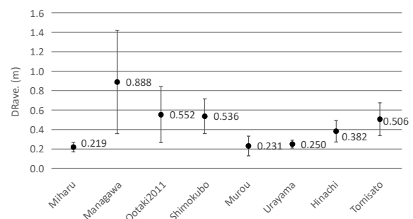
Fig. 1 Movable particle sizes of planned high water discharge at the downstream of dams.
