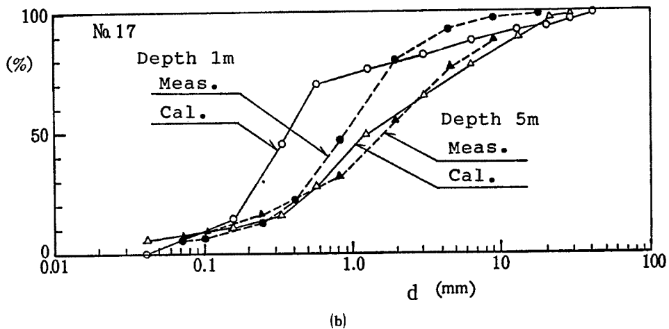
Fig. 15 (a), (b) Comparison between theoretical results and real ones on grain size distribution of bed materials.
