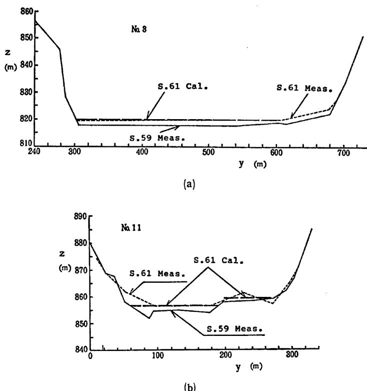
Fig. 14 (a), (b) Results on calculation of reappearance of sedimentation in lateral direction.
