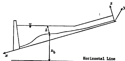
Fig. 8 Coordinate system.
