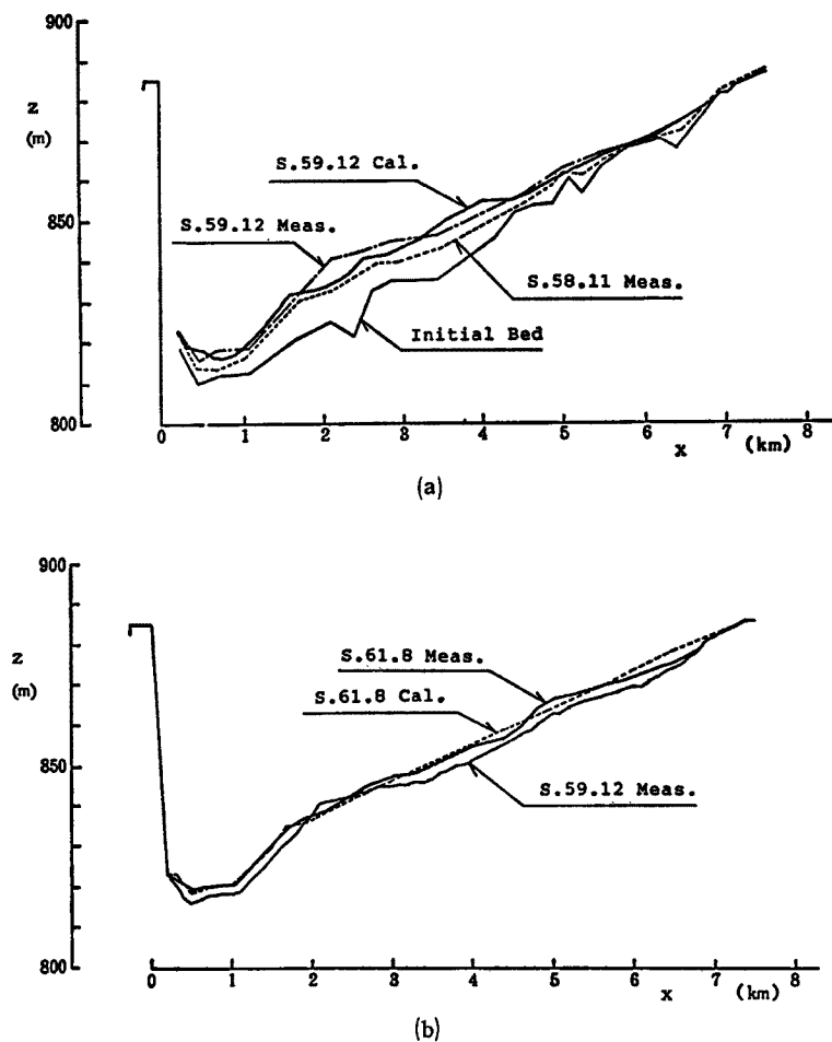
Fig. 13 (a), (b) Results on calculation of reappearance of sedimentation.
