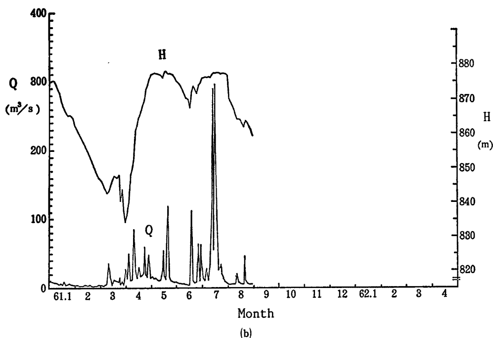
Fig. 4 (a)-(b) Discharge and water level.
