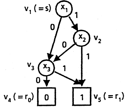
Figure 2: A BDD.
