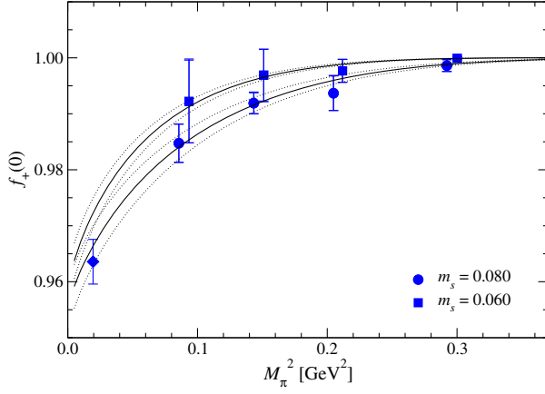
FIG. 7. Chiral extrapolation of f_+(0) as a function of M_\pi^2 . Solid circles and squares show our data at m_s = 0.080 and 0.060 . The blue diamond is the value extrapolated to the physical point (m_{l,\text{phys}}, m_{s,\text{phys}}) . We note that the physical strange quark mass m_{s,\text{phys}} (diamond) is slightly off the simulated values (solid lines).
