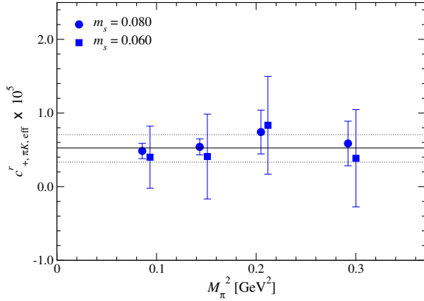
FIG. 9. Effective value c_{+, \pi K, \text{eff}}^r as a function of M_\pi^2 . Squares are slightly shifted along the horizontal axis for clarity. The solid and dotted lines show c_{+, \pi K}^r obtained from the NNLO chiral fit and its uncertainty.
