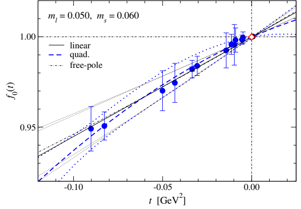
FIG. 6. Same as Fig. 4, but for (m_l, m_s) = (0.050, 0.060) .
