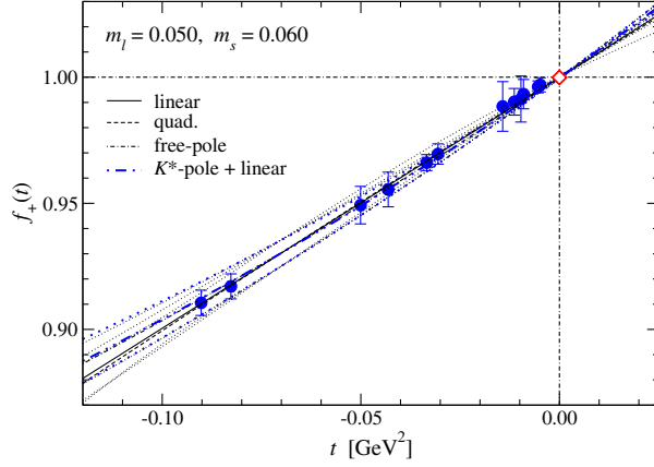
FIG. 6. Same as Fig. 4, but for (m_l, m_s) = (0.050, 0.060) .
