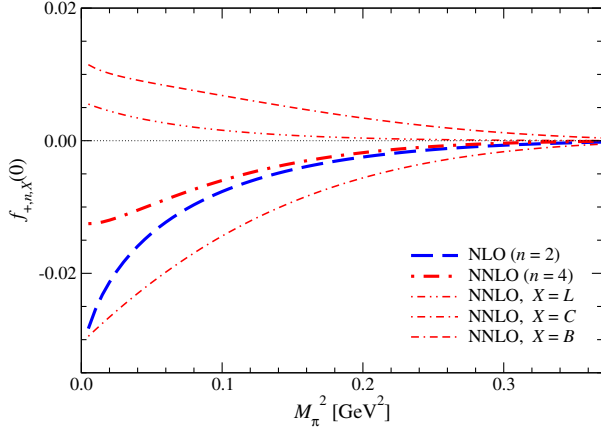
FIG. 8. LEC-(in)dependent NLO and NNLO contributions to f_{\pi,n\chi}(0) . Thick dashed and dot-dashed lines are the NLO and NNLO contributions, whereas the NNLO terms, f_{+,4,L}(0) , f_{+,4,C}(0) and f_{+,4,B}(0) , are plotted by the thin dot-dot-dashed, dot-dashed and dot-dashed-dashed lines, respectively.
