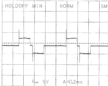
(a) stimulate pulse (ANALOG PROCESS)
