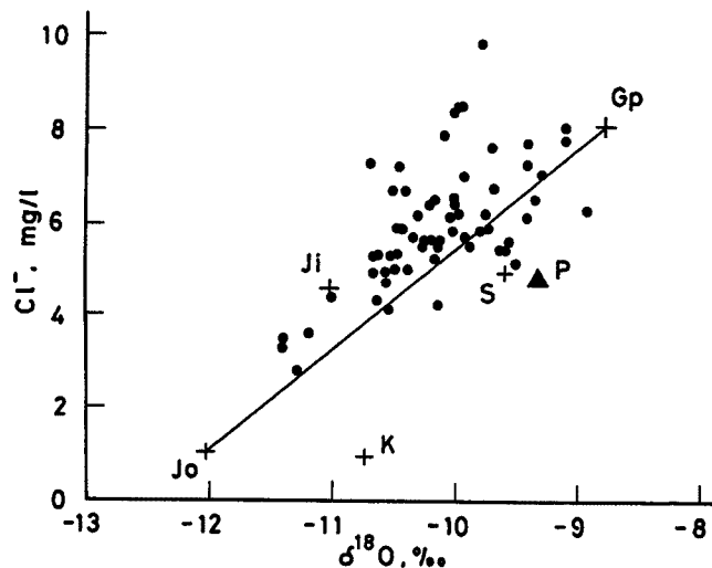
Fig. 6. Plot of \delta^{18}\text{O} versus chloride content for Joganjigawa Fan water samples. The symbols are the same as given in Fig. 4.
