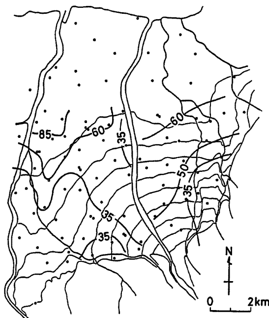
Fig. 9. Map showing bicarbonate contents (ppm) of ground water in the Joganjigawa Fan.
