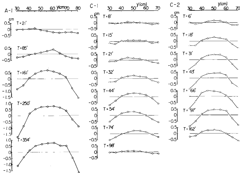
Fig. 16 Examples of bell-shaped cross section of the bed averaged longitudinally.
