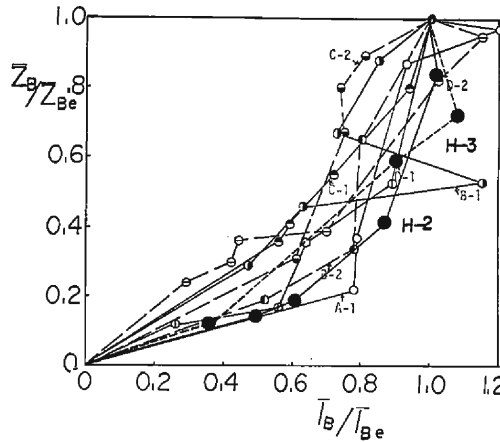
Fig. 10 A nondimensional relationship between the wave length and the wave height in the development process.
