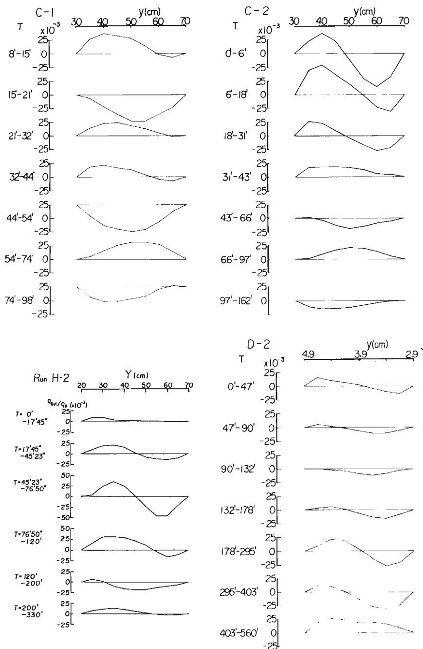
Fig. 17 Changes of averaged direction of sediment movement, q_{By}/q_{Bx} , in the development process.
