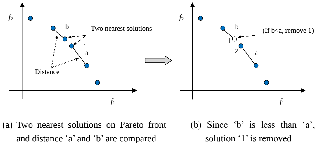
Fig. 5.6. Truncation Operator used in SPEA2
