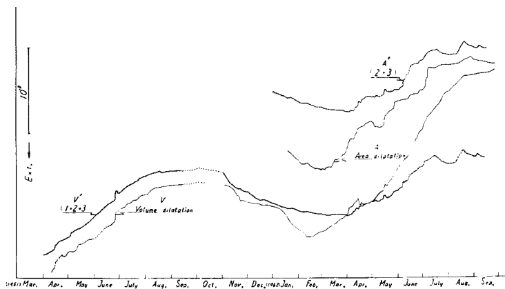
Fig. 3 Variations of the volume and area dilatations
