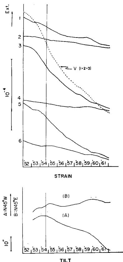
Fig. 4 Secular variations of the linear strains(—), volume dilatation (---) and the ground-tilts
