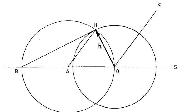
Fig. 1-5. Schematic representation of Laue condition.
