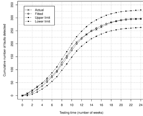
Fig 1 : Estimated expected number of faults detected, \hat{E}[N(i)] , and the 95% confidence limits for DS2.
