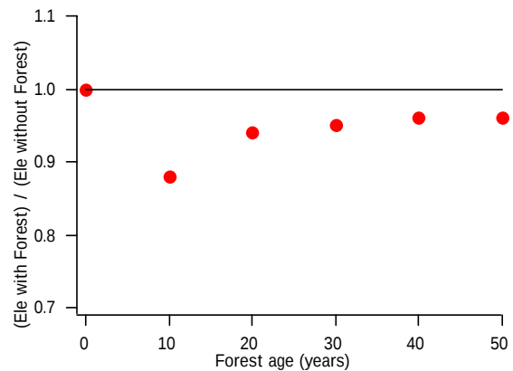
Fig.5 Relation of Reduction rate of maximum tsunami height and Forest years
