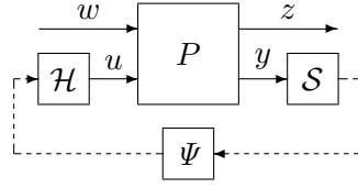
Figure 1. Sampled-data system \Sigma_{\text{SD}} .
