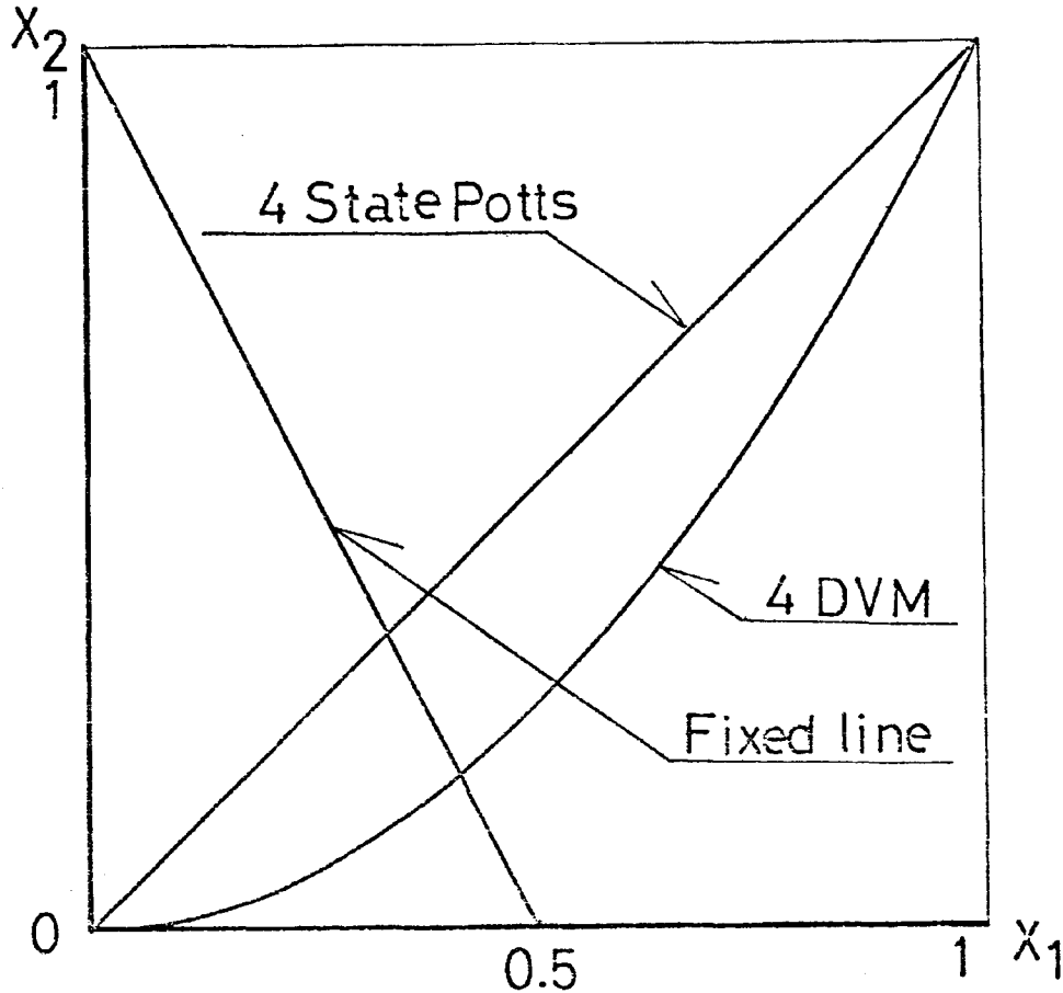
Fig. 4. The free energy of the four-state model is fixed by the duality transformation along the line x_2 = 1 - x_1 . The two lines representing the four-state Potts model ( x_1 = x_2 ) and the four-state discrete vector model (4DVM, x_2 = x_1^2 ) have common points with this line.
