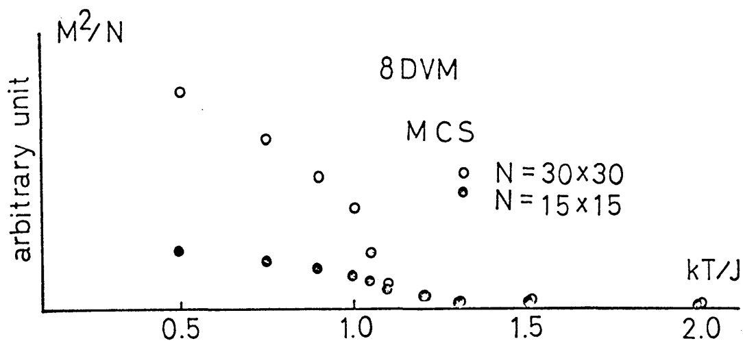
Fig. 15. (c) Susceptibility per spin divided by the temperature is equal to \langle M^2 \rangle because \langle M \rangle = 0 if kT/J \geq kT_c/J \simeq 0.6345 for 8DVM. The system size dependence of \langle M^2 \rangle/N below kT/J \simeq 1.15 implies the very large value in the limit N \rightarrow \infty .
