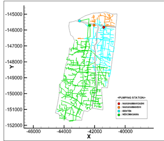
Fig. 2 Pipe connectivity analysis result
