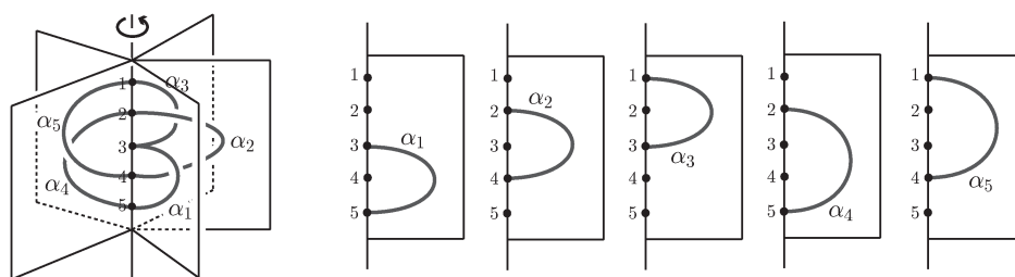
Figure 1: An arc presentation of the trefoil knot
