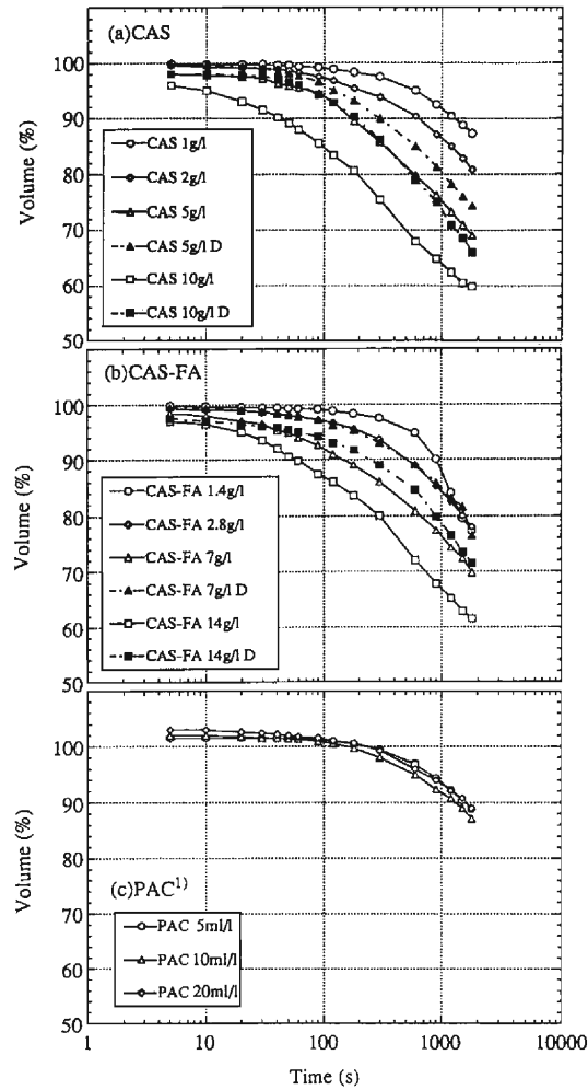
Fig. 3. Sedimentation characteristics of waste slurry A with flocculants.
