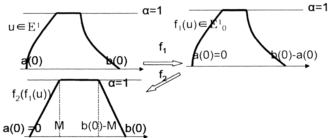
Fig. 5. Fuzzy mappings f_1 and f_2 .
