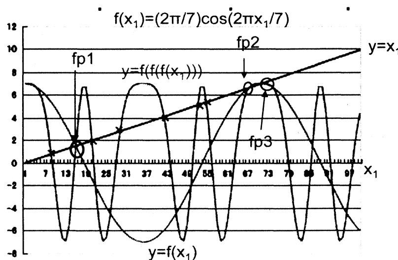
Fig.1. Function f(x_1) = (2\pi/7)\cos(2\pi x_1/7) has three fixed points and six
