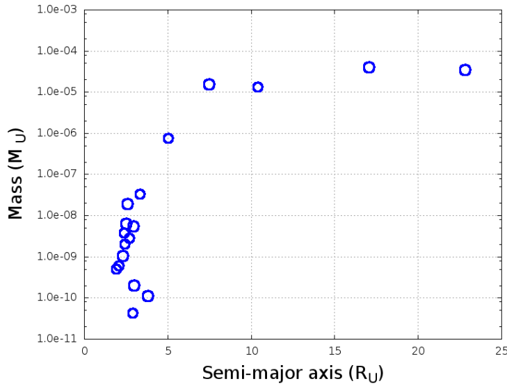
FIGURE 1.1: The mass distribution of the regular satellites orbiting around Uranus. The horizontal axis indicates the semi-major axes of the satellites normalized by the Roche limit and the vertical axis indicates the satellite mass normalized by the Uranian mass with log scale. The satellites are represented as circles. Satellites in the region from 5R_U to 23R_U are the five major satellites: Miranda, Ariel, Umbriel, Titania and Oberon in this order from the inner side.
