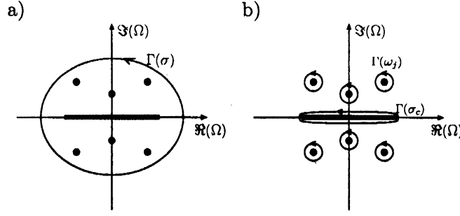
FIG. 1: Path of the Dunford integration
