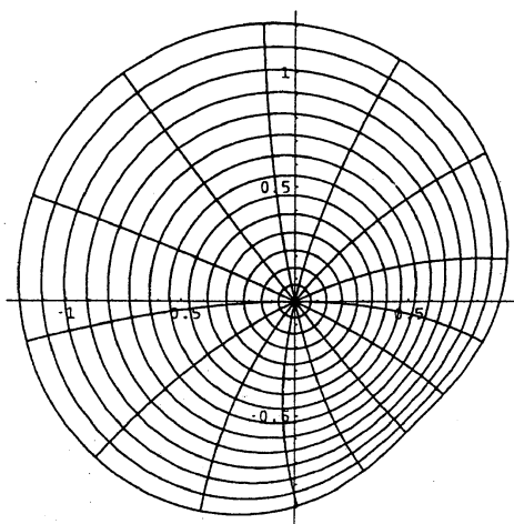
Figure 5: image of |z| \leq 1 by g(z) = z - \frac{1+i}{4\sqrt{2}}z^2
