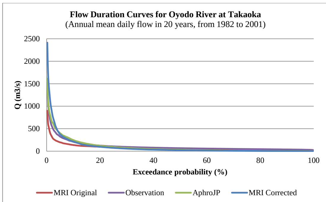
Fig. 6.12 Calendar-year flow duration curve of daily flow for Oyodo River at Takaoka
