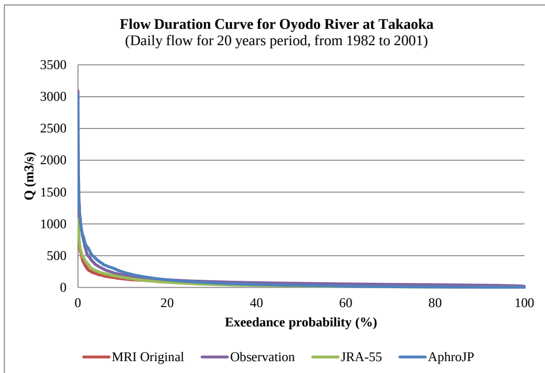
Fig. 6.6 Total period flow duration curve of daily flow for Oyodo River at Takaoka
