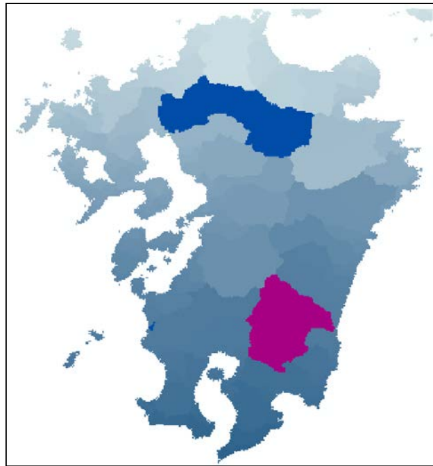
Fig. 6.1 Location of Chikugo River basin (blue) and Oyodo River basin (red) in Kyushu area, Japan
