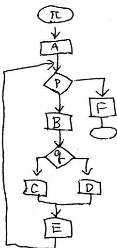
Goldstein - Neumann
