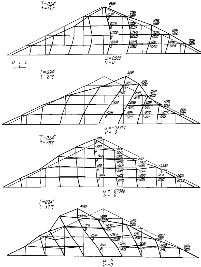
Fig. 6. Displacements due to the two-dimensional vibration by the external wave period 0.24 sec.
