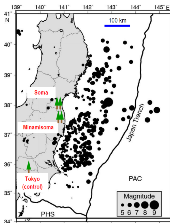
Figure 1. Three sites of tree sampling in Japan. Soma and Minamisoma were selected close to the hypocenter location of the mainshock and aftershocks exceeding a magnitude of 5 (black circles) within 24 h of the 11 March 2011 megathrust earthquake in northeast Japan. Tokyo was used as a control.
