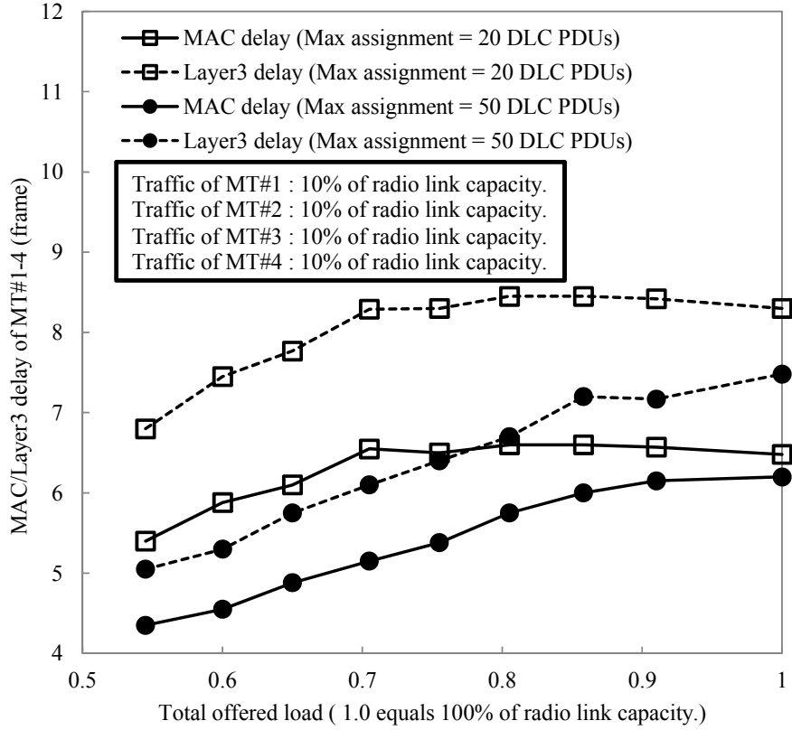
Fig. 3-19. MAC/Layer3 delay of MT#1-4 when only traffic of MT#0 is changed (Conventional, Case 2).
