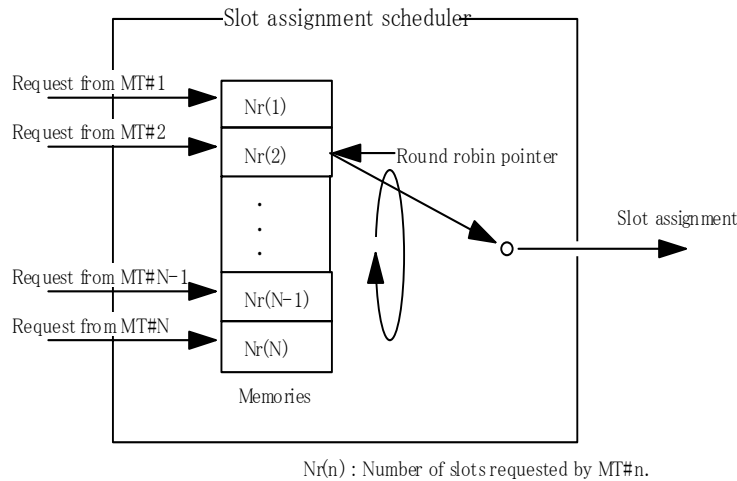
Fig. 3-7. Basic structure of SAS with conventional scheme.
