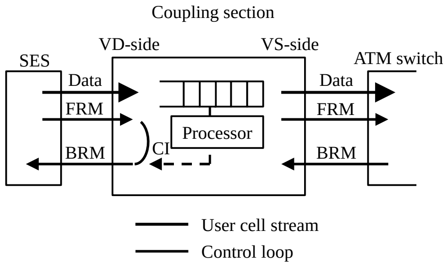
Fig. 4-1. VD/VS structure.
