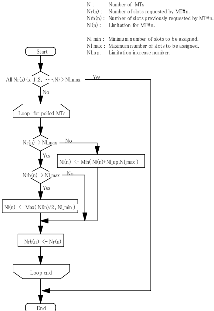
Fig. 3-12. Flow chart of usable slot size calculation.
