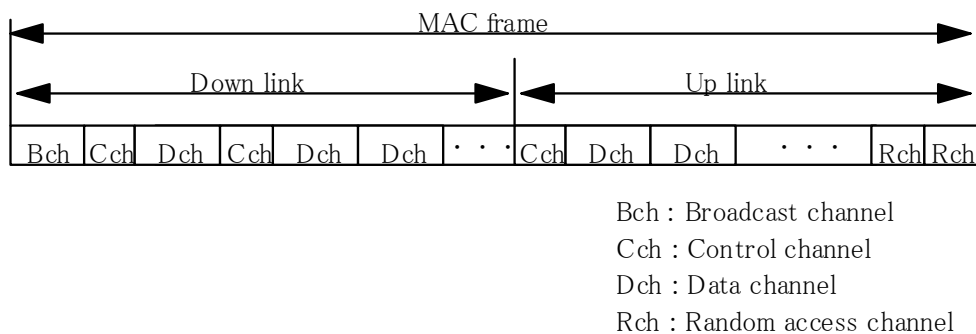
Fig. 3-2. Structure of MAC frame.
