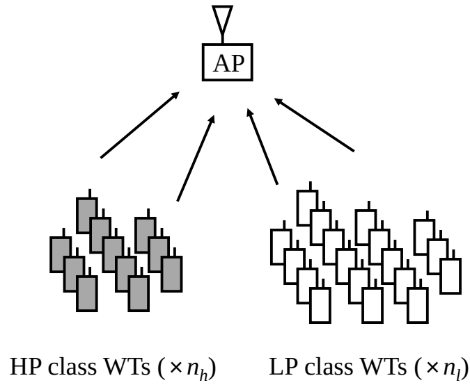
Fig. 6-12. Simulation model.
