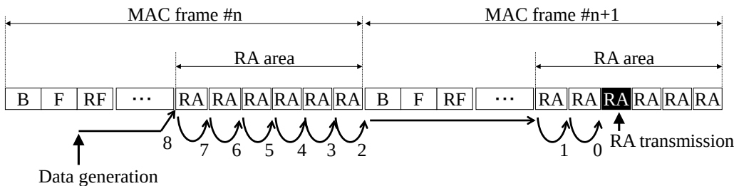
Fig. 6-6. Back-off in two MAC frame.
