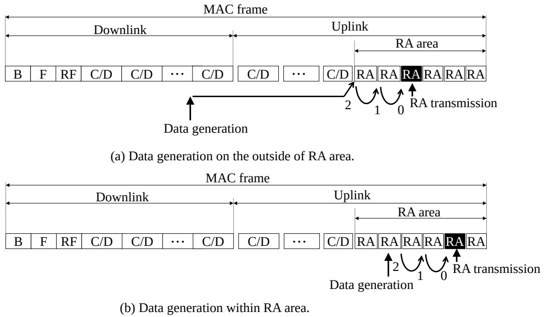
Fig.6-4. RA back-off procedure.
