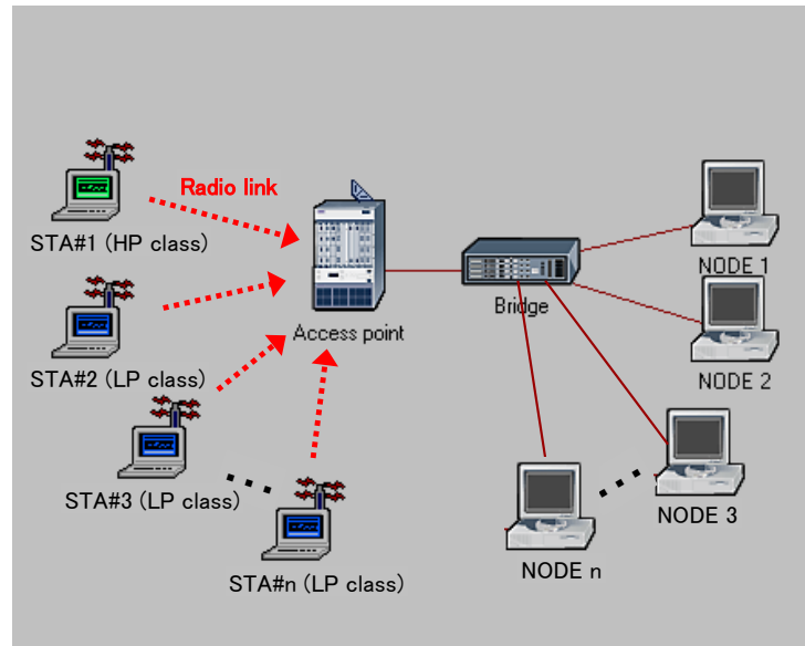
Fig. 5-5. n-STA simulation model (Model A).
