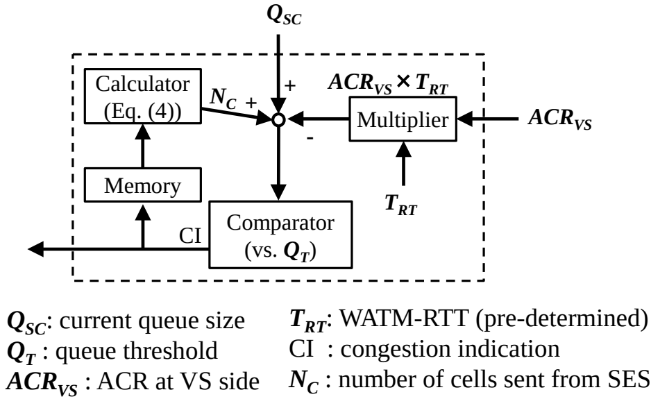
Fig. 4-5. Processor structure (proposed scheme).
