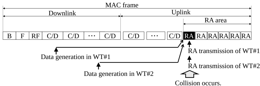
Fig. 6-5. RA transmission without back-off.
