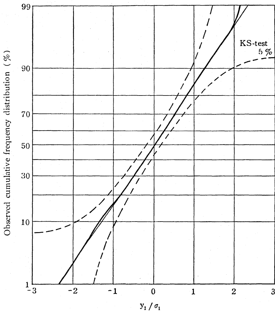
Fig. 7. Observed cumulative frequency distribution of the first component of the residual. ( t=t_f ).
