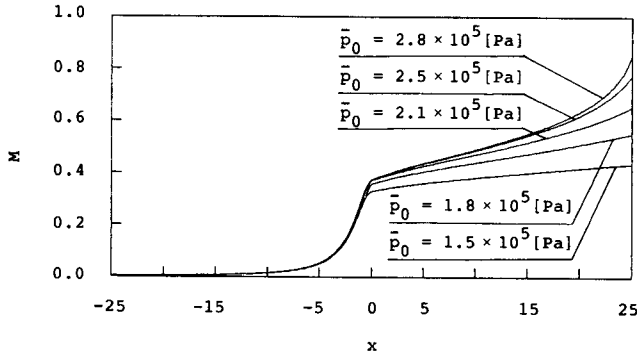
Figure 14 Variation of local gas-phase Mach number along nozzle axis with \bar{p}_0 as a parameter ( \bar{p}_e=1.0 \times 10^5 [\text{Pa}] and \nu=3 ). Note that the nozzle geometry given by Eq. (100) is adopted in this calculation.
