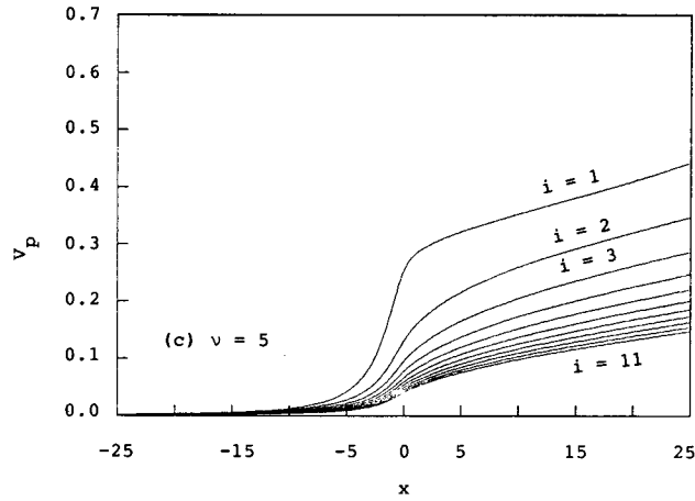
Figure 2 Variation of particle velocities along nozzle axis for \nu=1.0 (a), \nu=3.0 (b) and \nu=5.0 (c). Note that i is the size number to present the particle radius (see Table 2).
