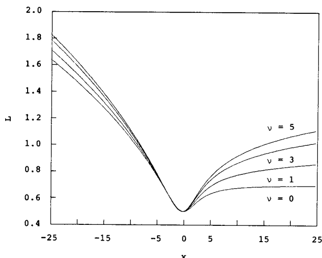
Figure 7 Nozzle geometry calculated according to pressure profile shown in Fig. 6. Note that \bar{p}_0 = 10.0 \times 10^5 [\text{Pa}] for the supersonic nozzle flow and \bar{p}_e = 1.0 \times 10^5 [\text{Pa}] , and that the gas-phase pressure in the mixture flow is taken to be equal to the ambient gas pressure ( p_e = 0.1 ).
