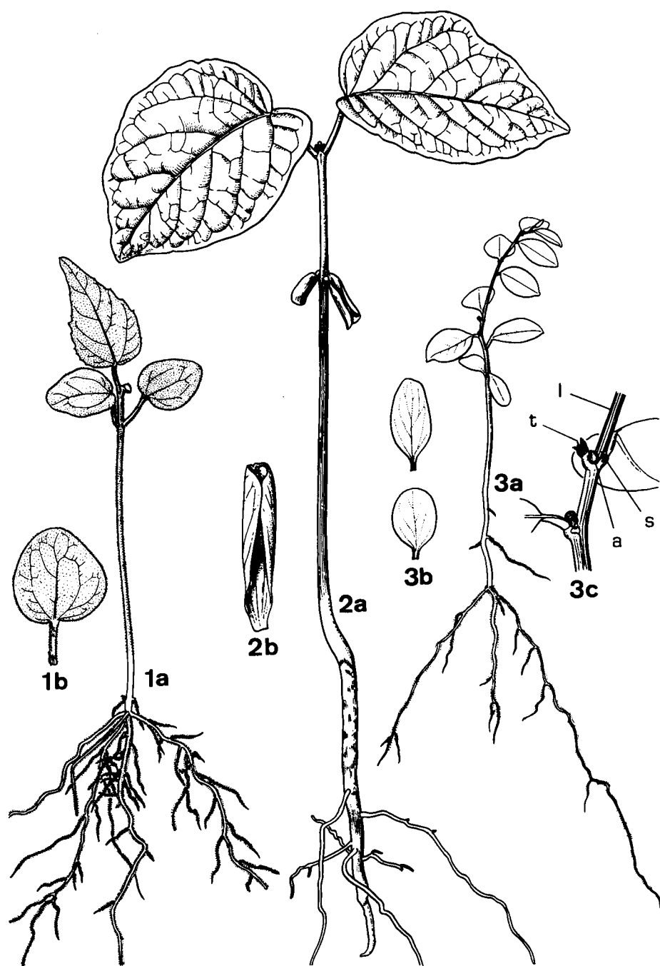
図-4 1. アカメガシワ Mallotus japonicus , 1a: habit ( \times 1 ), 1b: cotyledon ( \times 1.5 ) 2. シラキ Sapium japonicum , 2a: habit ( \times 1 ), 2b: old cotyledon, adaxial view ( \times 2 ) 3. コバンノキ Phyllanthus flexuosus , 3a: habit ( \times 1 ), 3b: cotyledons ( \times 2 ), 3c: apex of shoot, showing a dormant terminal bud and a lateral shoot ( \times 4 ). a: accessory bud, l: lateral shoot, s: stipule, t: terminal bud
