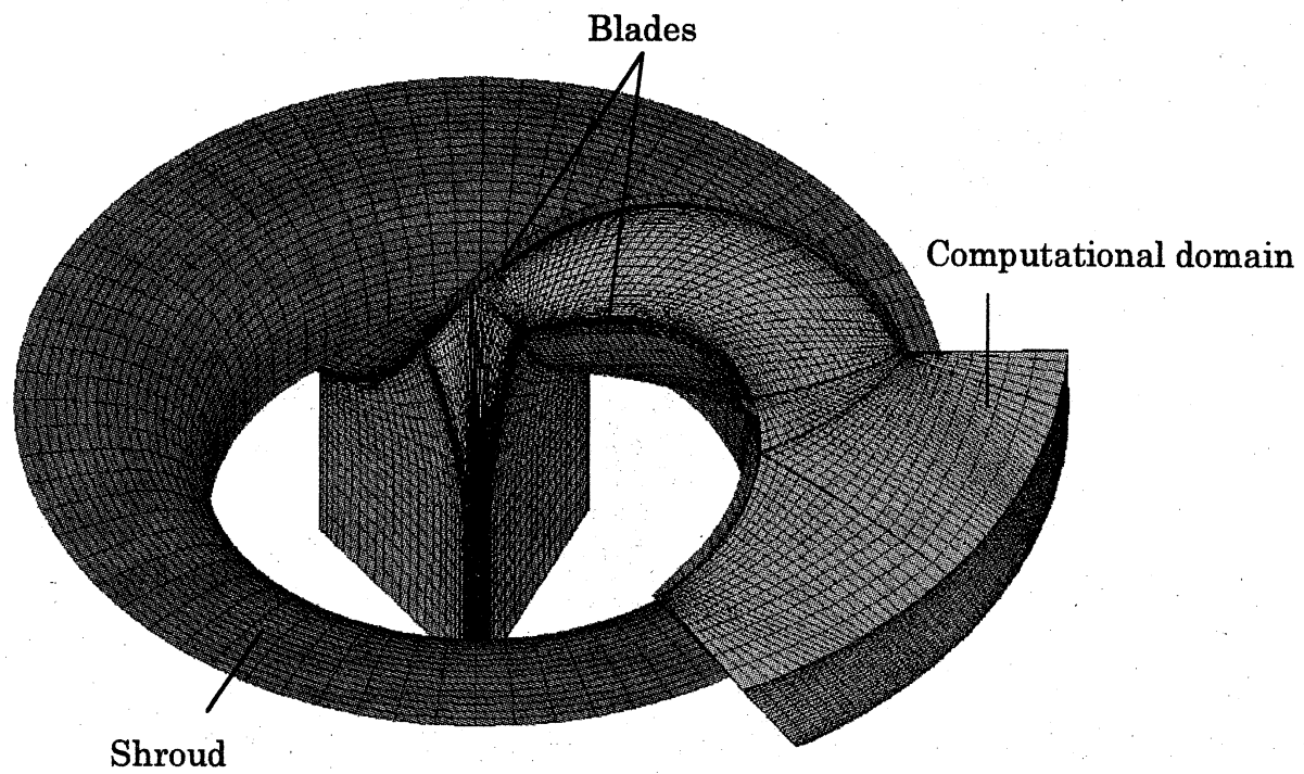
Fig.3 Computational domain of a flow analysis in the pump turbine
