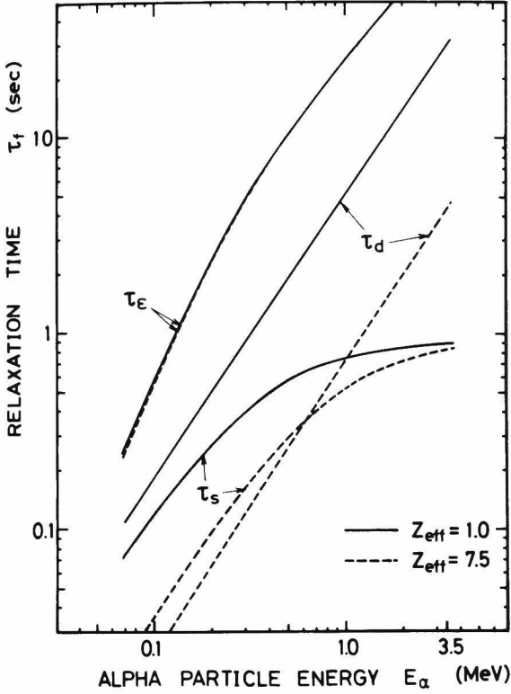
Fig.5.3. Relaxation times of the alpha particles with various energies in a pure DT plasma (solid curves) and in a highly contaminated plasma (broken curves), where T_e=8 KeV and n_e=1.0 \times 10^{20} \text{ l/m}^3 .
