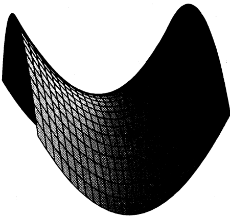
Figure 1: hyperbolic paraboloid
