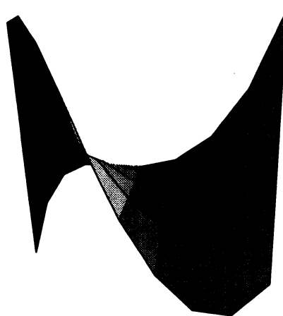
Figure 4: discrete Cayley surface
