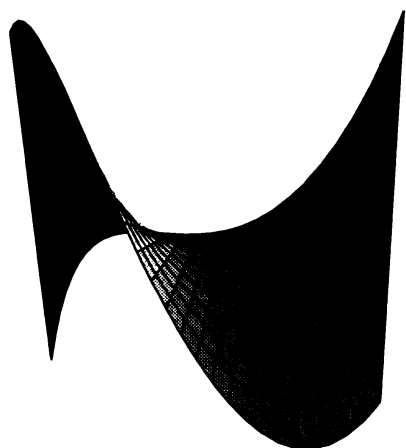
Figure 3: Cayley surface
