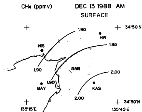
Fig. 9(a). Horizontal distribution of methane volume mixing ratio on the surface in the morning of 13 December 1988.
