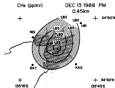
Fig. 8(b). Same as Fig. 8 (a), except for in the afternoon. The area of slanting lines where mixing ratio is higher than 1.80 ppmv expanded compared to Fig. 8 (a) in the morning.
