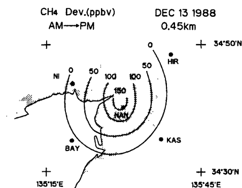
Fig. 12. Same as Fig. 11, except for 13 December 1988.
