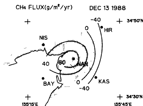
Fig. 15. Same as Fig. 14, except for 13 December 1988.
