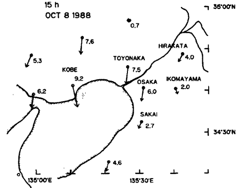
Fig. 2(b). Same as Fig. 4 (a), except for in the afternoon (15h).
