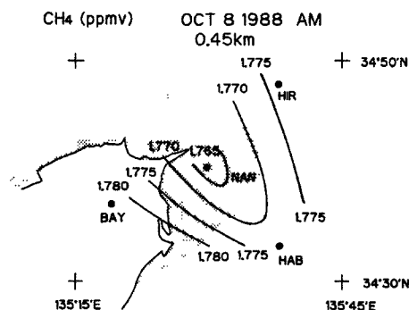
Fig. 10(a). Horizontal distribution of methane volume mixing ratio at the altitude of 0.45 km in the morning of 8 October 1988.
