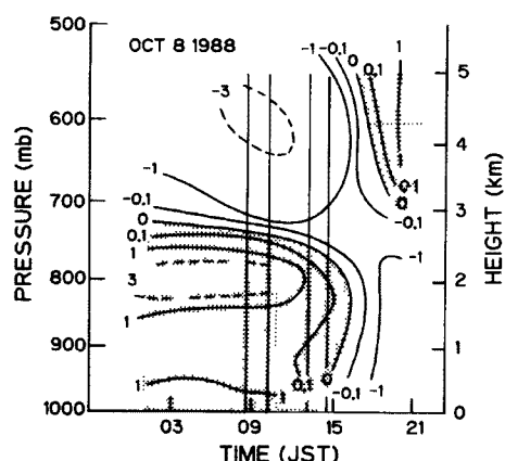
Fig. 17. Same as Fig. 16, except for on 8 October 1988.
