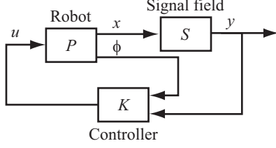
Fig. 2. Control system for source seeking.
