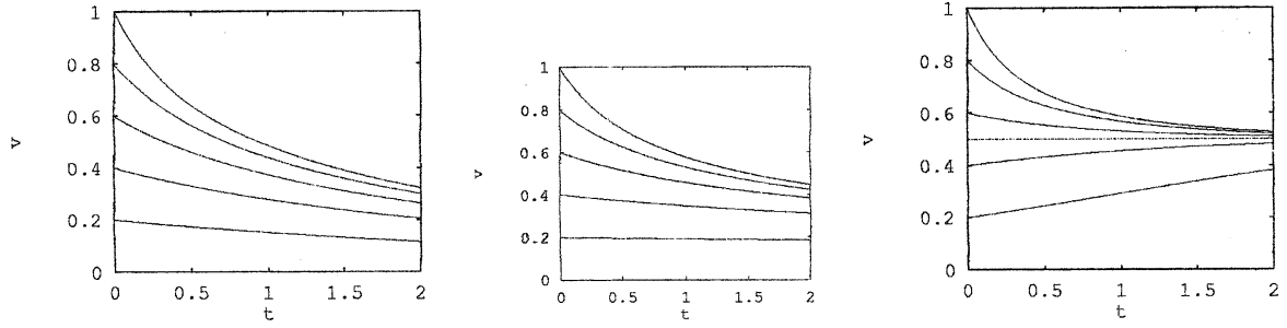
Figure 1: Evolution of homogeneous solutions, \beta < 0, \beta = 0, \beta > 0 , respectively
