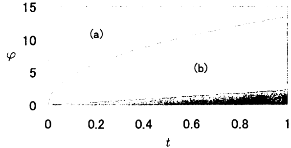
Figure 4: The region of pairs (t, \varphi) .
