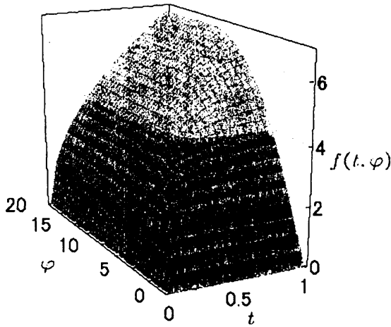
Figure 3: The form of the function f(t, \varphi) .
