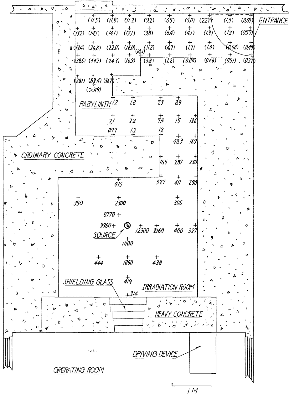
Fig. 7. Distribution of experimental dose rates in the irradiation room and the labyrinth (Normalized to February 15, 1961). The dose rates are given in units of r/hr, except those in parentheses in units of mr/hr.
