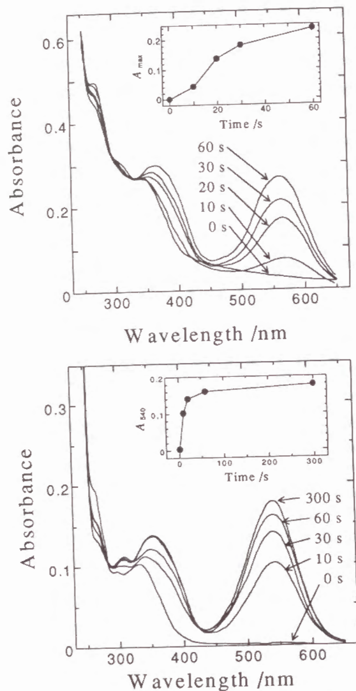
Figure 3. Absorption spectra under UV-light irradiation of M4Sp (a) and M7Sp (b) in the presence of DPPC vesicles. [peptide] = 8.5 \mu\text{M} . [DPPC] = 0.64 mM.
