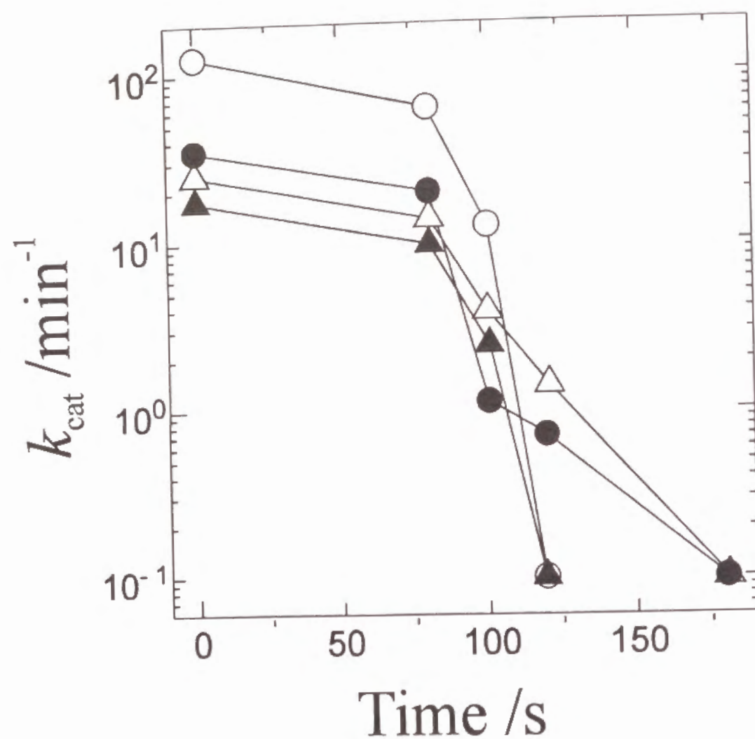
Figure 5. Thermostability of purified \beta -D-galactosidases. The specific activity is plotted against incubation times of 80 s, 100 s, 120 s, and 180 s. \circ , sample obtained from the cells of strain DH5 \alpha grown without nonnatural amino acid; \bullet , \triangle and \blacktriangle , samples obtained from the cells of strain DH5 \alpha grown in the presence of pyrAla, antAla, and napAla, respectively.
