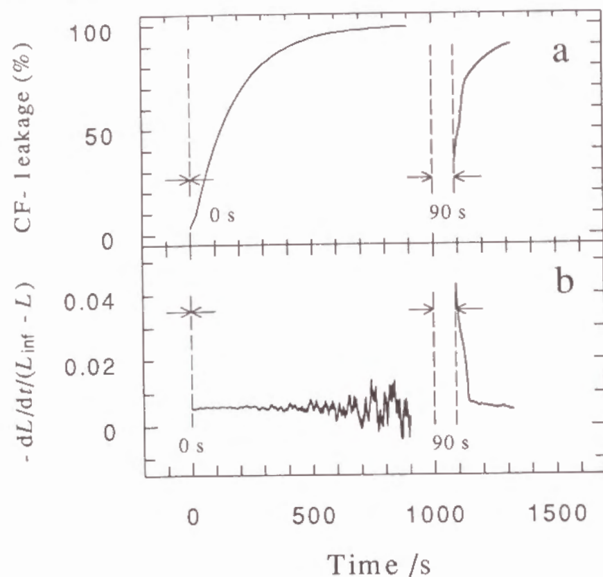
Figure 3. CF leakage from DPPC vesicles induced by MSp at 15 °C. a : the percentage of CF leaked from the vesicles. b : the rate constant of CF leakage. dL/dt was calculated by numerical differentiation of the experimental data. Left: without UV-light irradiation. Right: UV-light irradiation for 90 s.
