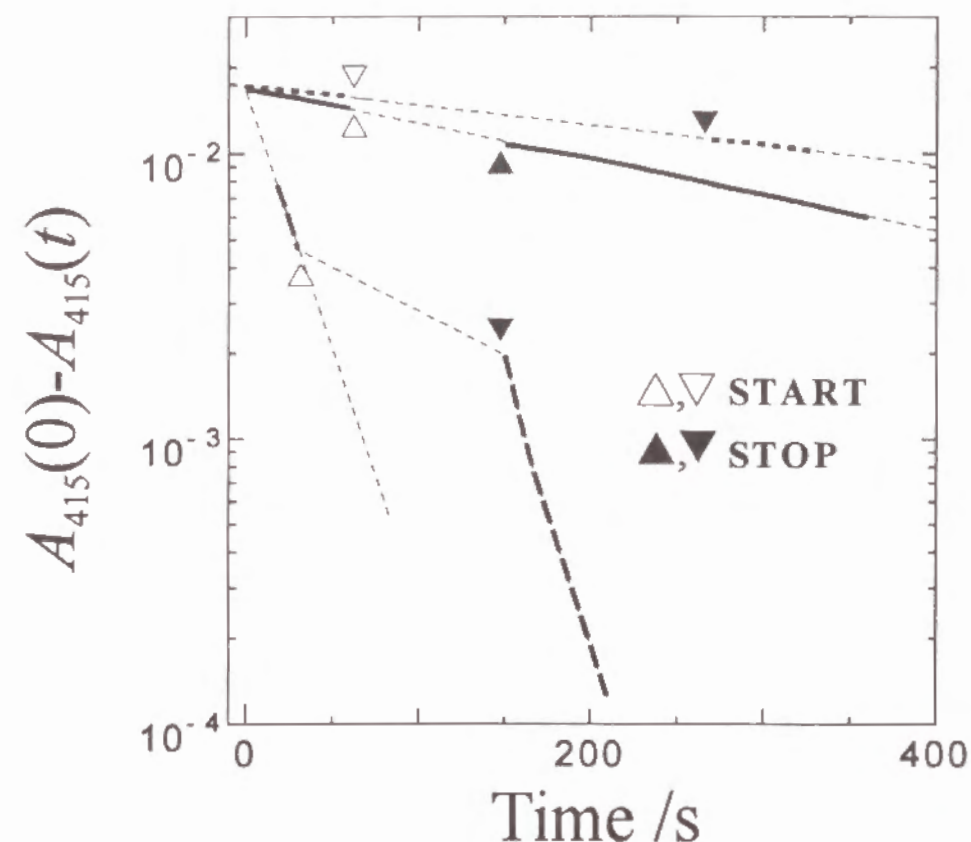
Figure 7. Reduction kinetics of native and mutant cytochromes c with or without light irradiation. (-----), PGL-Cytc; (—), native cytochrome c ; (— · —), PYR-Cytc. Light irradiation was started at the time shown by open triangles (△, ▽), and was stopped at the time indicated by filled triangles (▲, ▼). During light irradiation, the reduction reaction could proceed as represented by thin broken lines (---).
