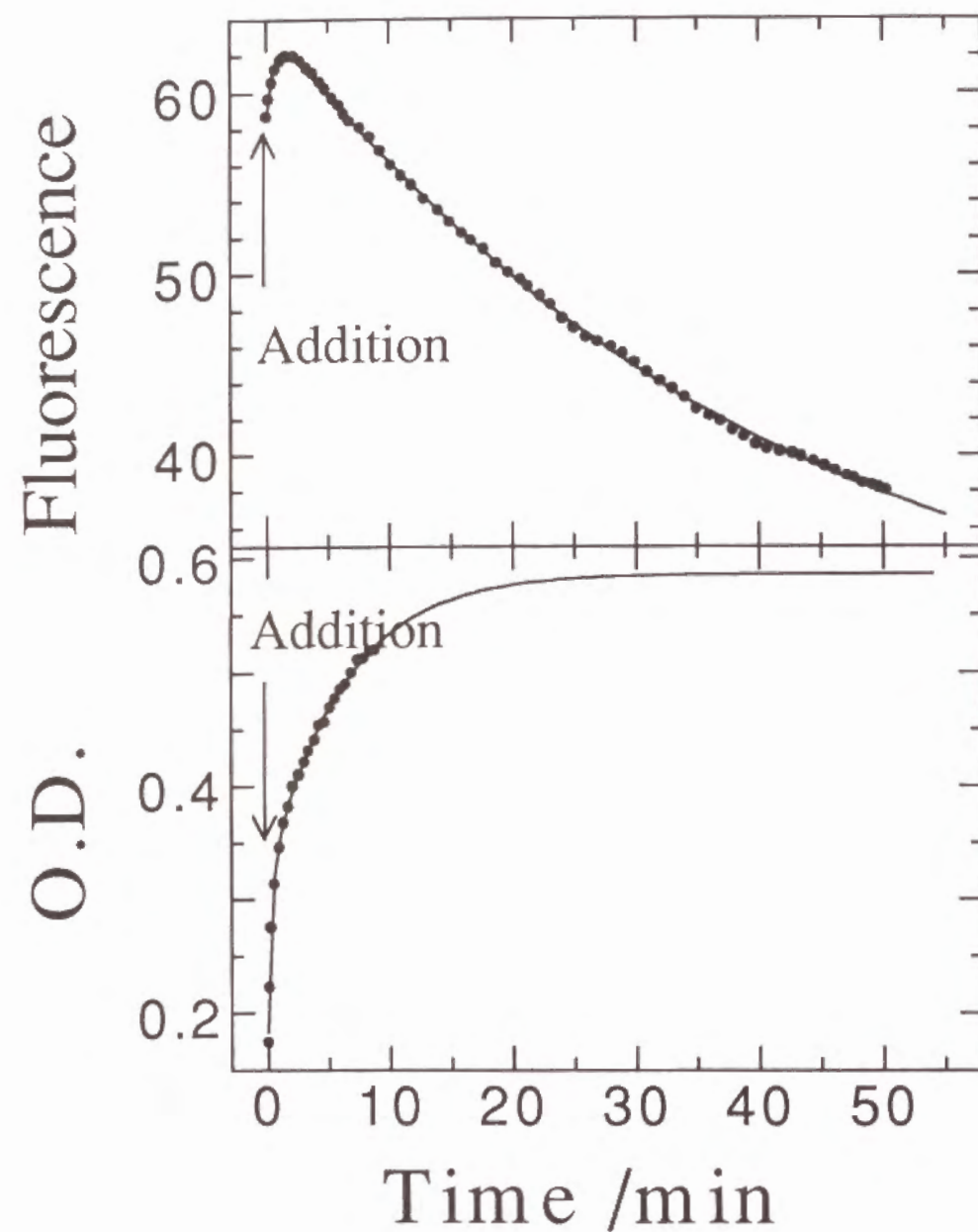
Figure 6. Changes of fluorescence intensity of Quin 2-encapsulated DPPC vesicles (top) and of absorption at 290 nm (bottom) on addition of Ant-AMPA (1.65 \mu M).
