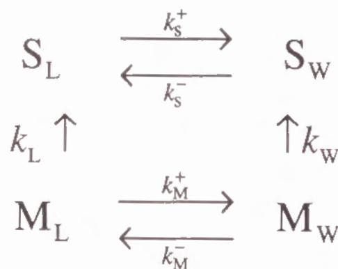
Figure 5. Thermal decoloration pathways of MSp in the presence of vesicles. The subscripts L and W represent the lipid membrane phase and the aqueous phase, respectively. S and M represent MSp in the form of spiropyran and merocyanine, respectively.
