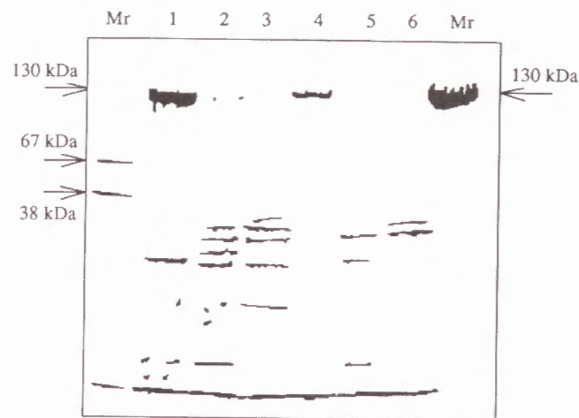
Figure 3. The SDS-PAGE profile of produced β-D-galactosidases. β-D-Galactosidase was obtained from various strains without nonnatural amino acid. Mr, Marker; lanes 1 and 4, DH5α strain harboring pUC19Z; lanes 2 and 5, DH5α strain harboring pUC19; lanes 3 and 6, DH5α without transformation. Lanes 1, 2, and 3, 20 µg protein each; lanes 4, 5, and 6, 10 µg protein each.
