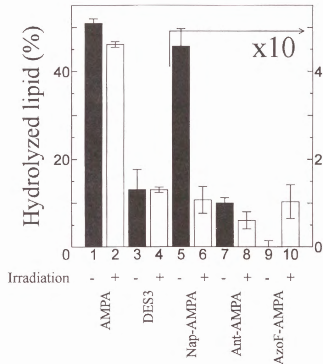
Figure 7. Effect of UV-light irradiation on hydrolytic activity of AMPA, DES3, and mutant PLA 2 s. The ordinate represents the amount of hydrolyzed lipid molecules after 60 min. Without UV-light irradiation, . With UV-light irradiation, . Standard errors of the mean (SEMs) are shown as I-bars.
