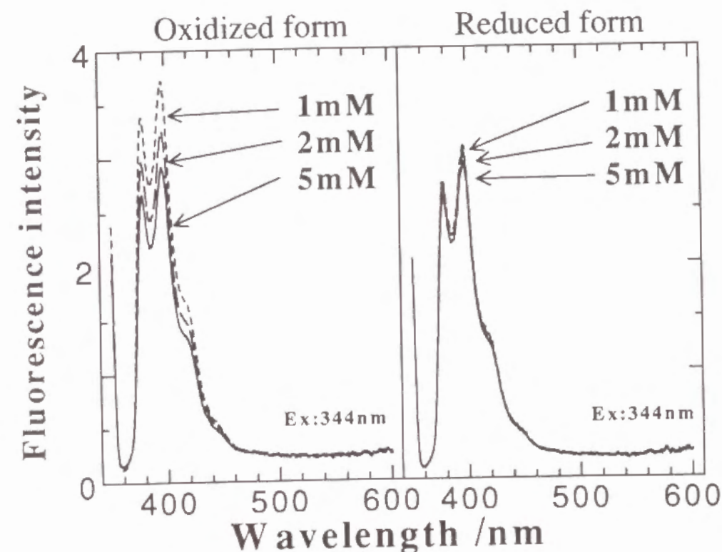
Figure 1. Fluorescence quenching of oxidized and reduced form of PYR-Cytc. Left: fluorescence spectra of ferricytochrome c in the presence of 1 mM, 2 mM, and 5 mM of acrylamide. Right: fluorescence spectra of ferrocyanochrome c in the presence of acrylamide. PYR-Cytc was completely reduced by adding 1 % (v / v) of 2-mercaptoethanol followed by standing for 24 h at room temperature in the dark and subsequent gel permeation chromatography on a Sephadex G-25 (fine grade) column with potassium phosphate buffer solution (pH 7.2) as eluent. Excitation wavelength was 344 nm.
