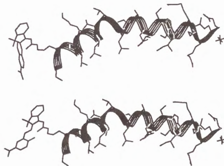
Figure 6. 3D ribbon drawing of melittin carrying a chromophoric group in spiropyran form (top) or merocyanine form (bottom). Backbone and side chains are superimposed on the ribbon. Ribbon drawings were created from the X-ray crystallographic data stored in the Protein Data Bank at BNL, USA, by using MAGE Version 2.5.
