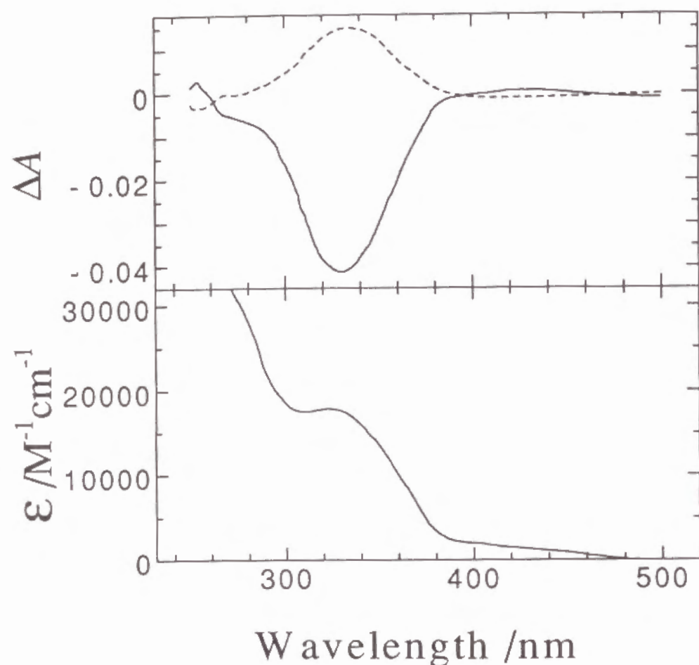
Figure 3. Photoisomerization of AzoF-AMPA monitored by UV spectroscopy. The bottom spectrum is AzoF-AMPA in Tris-HCl buffer (10 mM, pH 7.8). Difference spectra between after and before UV-light irradiation (—) and between after and before visible-light irradiation (---) are shown in the top figure. Photoisomerization from trans - to cis - configuration was induced by UV-light irradiation using a UV31 optical filter and a solution filter of nickel(II) sulfonate. Visible-light irradiation using an L39 optical filter was used for the cis to trans isomerization. Concentration of AzoF-AMPA was 1.13 \mu M.
