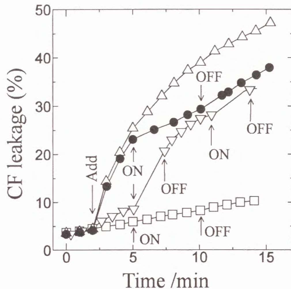
Figure 4. CF leakage from DPPC vesicles induced by the addition of M1Sp ( \square ), M4Sp ( \nabla ), and M7Sp ( \bullet ). Arrows of Add, ON, and OFF represent the addition of the peptide, UV-light irradiation, and visible-light irradiation, respectively. ( \triangle ) represents the effect of M7Sp addition without UV-light irradiation. [DPPC] = 60 \mu\text{M} . [peptide] = 0.2 \mu\text{M} . Temperature = 25 ^{\circ}\text{C} .
