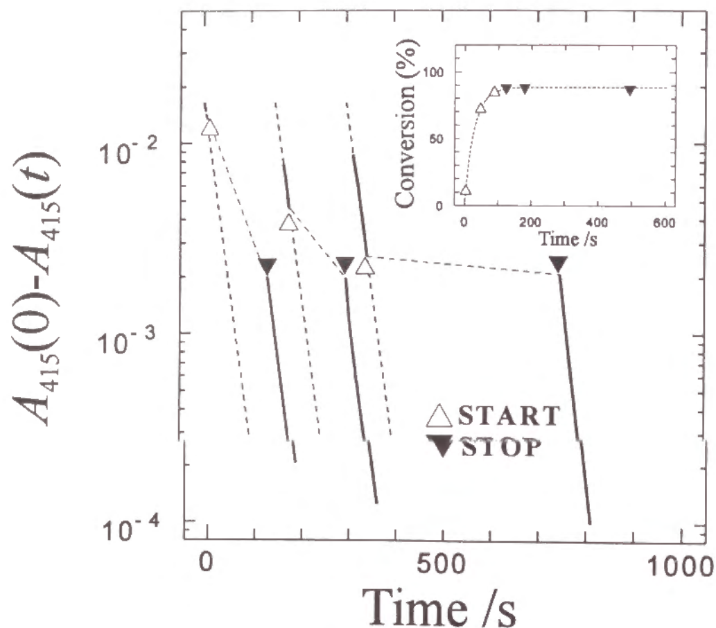
Figure 8. Dependency of the reduction reaction of PYR-Cytc on duration of light irradiation. (—), the absorbance change on keeping in the dark. The light irradiation was started at the time indicated by open triangles ( \triangle ), and was stopped at the time indicated by filled triangles ( \blacktriangledown ). The thin broken lines (---) represent reduction reactions during light irradiation. The inset shows the calculated time-conversion (%) curve of reduction of PYR-Cytc by light irradiation.
