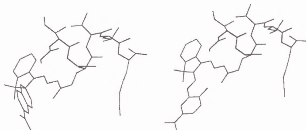
Figure 1. 3D wire frame drawing of melittin fragment carrying spiropyran. Backbone structure is illustrated by the wire frame model. Side chains are drawn in stick model. (Left) spiropyran form, (right) merocyanine form.
