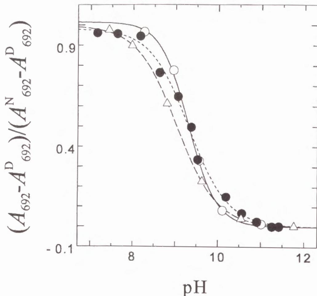
Figure 4. Alkaline transition of the native cytochrome c (●), PYR-Cytc (△) and fully N^{\epsilon} -amidinated cytochrome c (○). The protein concentration was 40 \mu M. The titration was monitored by absorbance change at 692 nm at 25 °C.
