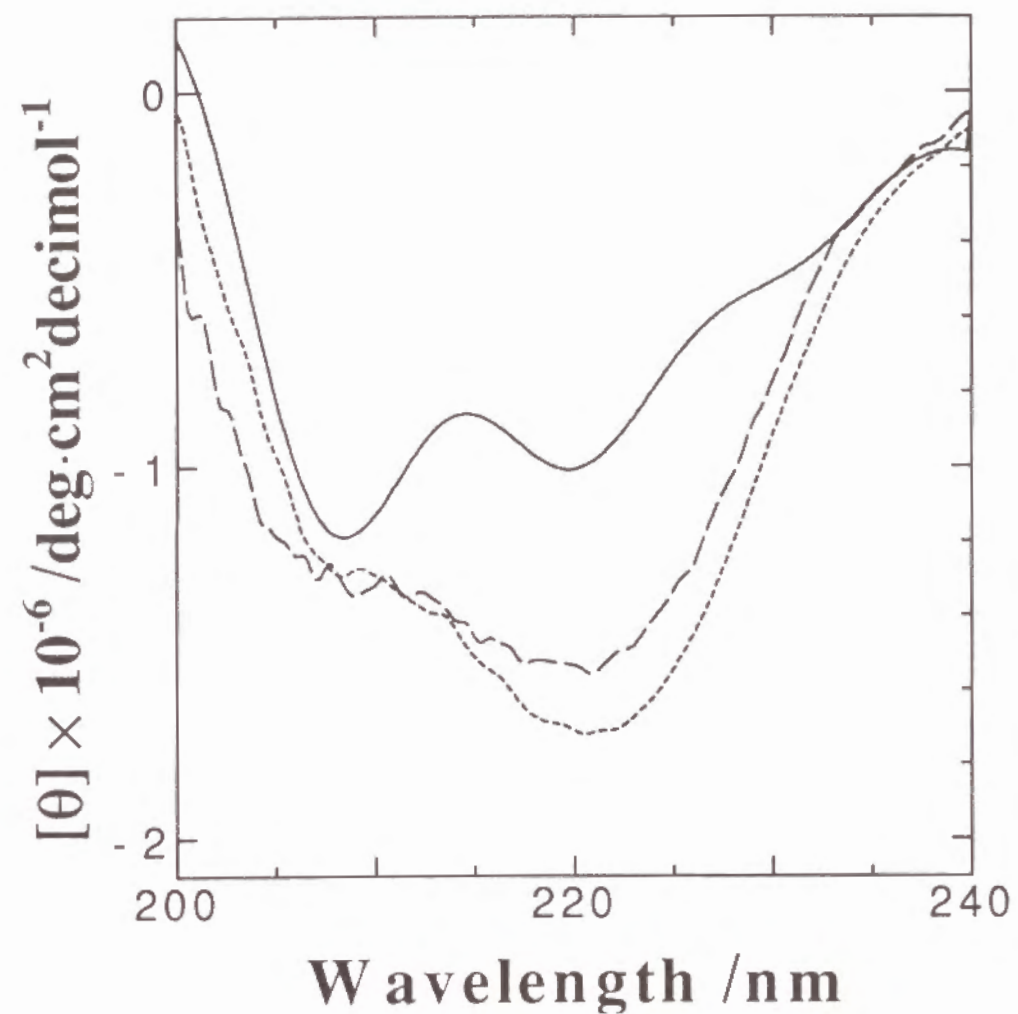
Figure 4. Circular dichroism spectra of mutant cytochromes c (200-240 nm region). (—), PYR-Cytc; (.....), native cytochrome c ; (---), PGL-Cytc. Concentration of each cytochrome c was 1.10 \mu M.
