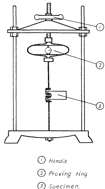
Fig. 10. Loading apparatus
