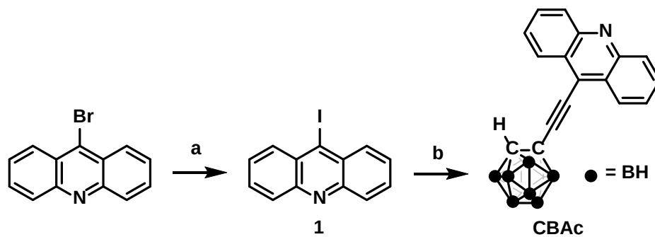
Scheme 1. Synthetic route of CBAc a
